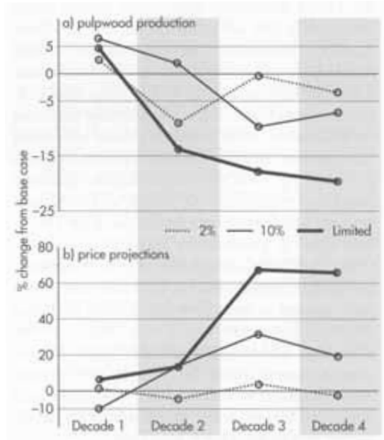
Fig. 2. Projections of softwood pulpwood production (a) and prices (b) with the FASOM model, with percentage changes relative to the FASOM base case for the three alternative scenarios.
