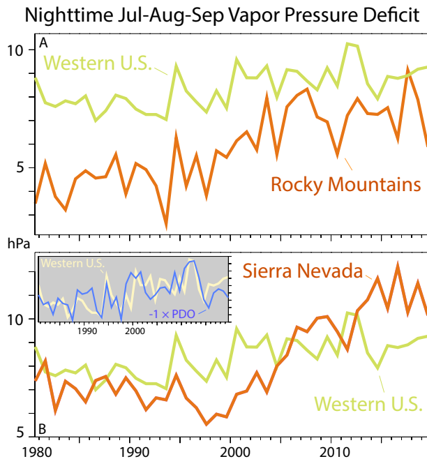
Figure 4. Summer-nighttime averaged vapor pressure deficit, 1980–2019. The western US curve shows the study region average. The Sierra Nevada and Rocky Mountain curves illustrate averages over these region's maxima, defined by increases between the recent (2010–2019) and earlier (1980–1999) periods >50% of the earlier period mean. The panel (b) inset shows the western US curve with summertime (July–August–September) values of the Pacific Decadal Oscillation (PDO) index (normalized to unit standard deviation).
