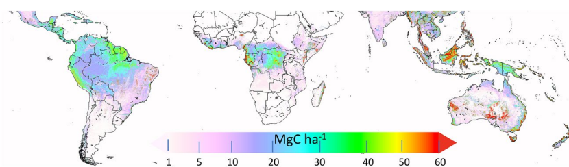
Figure 18. The uncertainty map for the above ground carbon shown in Figure 3. The uncertainty map is derived from a Bayesian approach described in Appendix A.1. The error is given at the 1-km pixel level (S. S. Saatchi et al., 2011).
