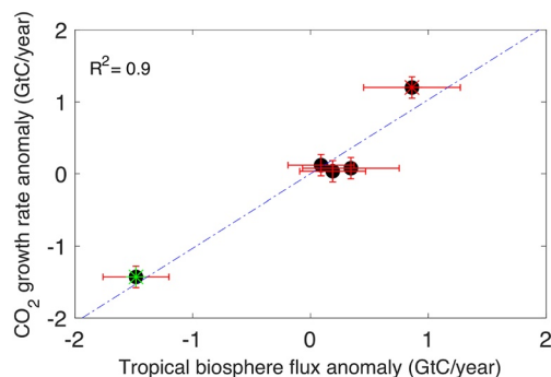
Figure 8. The relationship between atmospheric CO 2 growth rate anomaly (GtC/year) and the tropical biosphere flux anomaly (GtC/year) constrained by satellite column CO 2 observations, GOSAT data (red/black symbols) are shown for 2010–2013 and OCO-2 data (green hash symbols) is for 2015. GOSAT, Greenhouse Observation SATellite; OCO-2, Orbiting Carbon Observatory 2; SIF, solar induced chlorophyll fluorescence.
