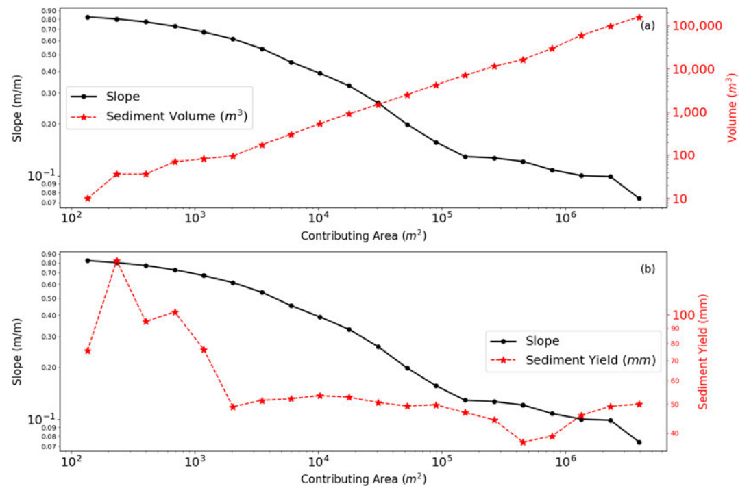
Figure 9. Slope-area curve compared to (a) the volume of sediment passing through each pixel and (b) the sediment yield at each pixel.
