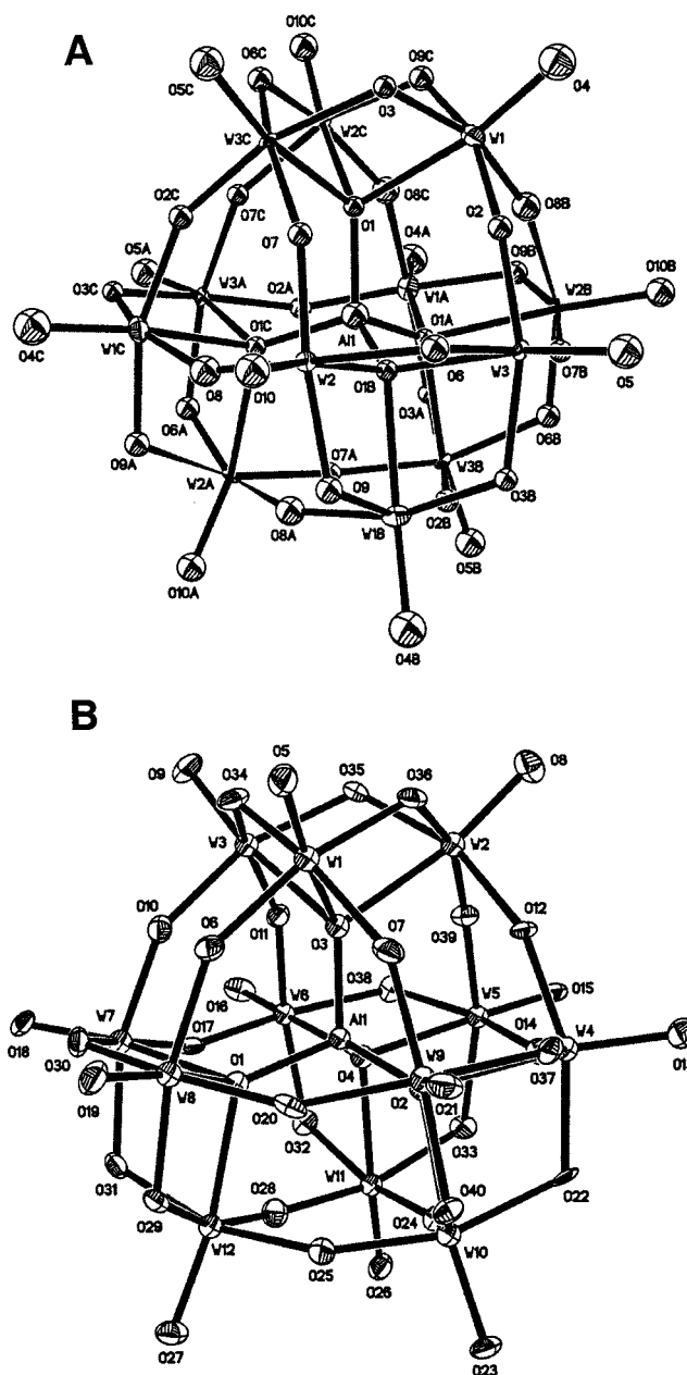
Figure 5. Thermal ellipsoid plot showing \alpha\text{-}[\text{AlMn}^{\text{III}}(\text{OH}_2)\text{W}_{11}\text{O}_{39}]^{6-} (A) and \alpha\text{-}[\text{AlCo}^{\text{II}}(\text{OH}_2)\text{W}_{11}\text{O}_{39}]^{7-} (B). Thermal ellipsoids are drawn at 80% probability in (A) and 30% probability in (B). In the solution of the structure of \alpha\text{-}[\text{AlMn}^{\text{III}}(\text{OH}_2)\text{W}_{11}\text{O}_{39}]^{6-} , each addendum-atom site was assigned 1/12 Mn character and 11/12 W character, and in the solution of the structure of \alpha\text{-}[\text{AlCo}^{\text{II}}(\text{OH}_2)\text{W}_{11}\text{O}_{39}]^{7-} , each addendum-atom site was assigned 1/12 Co character and 11/12 W character (see Experimental Section). For clarity, all W/Mn sites in (A) and all W/Co sites in (B) are labeled as W only.
