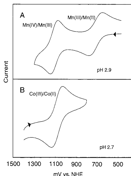
Figure 4. Cyclic voltammograms showing successive 1e − oxidations of α-[AlMn II (OH 2 )W 11 O 39 ] 2− to α-[AlMn III (OH 2 )W 11 O 39 ] 6− and α-[AlMn IV (OH 2 )W 11 O 39 ] 5− (A) and the 1e − oxidation of α-[AlCo II (OH 2 )W 11 O 39 ] 7− to α-[AlCo III (OH 2 )W 11 O 39 ] 6− (B).
