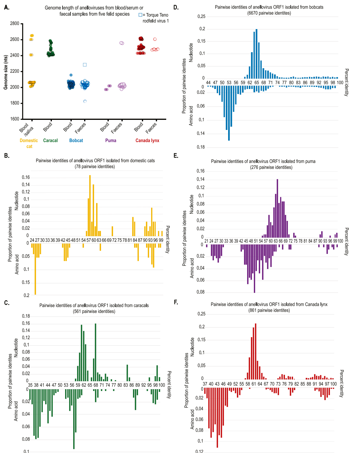
Fig. 1. Pairwise distributions of anelloviruses from each species show high within host diversity. A) Plot showing genome sizes of feline derived anelloviruses recovered from the five host species (this study and previously documented) and the different sample types. B–F) Pairwise distribution plots of anellovirus ORF1 nucleotide and amino acid sequences for the five feline species from which anelloviruses were recovered in this and previous studies.
