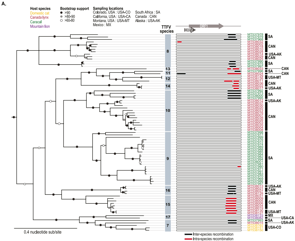
Fig. 4. Three anelloviruses recovered from bobcat and puma faecal samples appear to be derived from prey animals. A) Recombination free maximum-likelihood phylogeny of the anelloviruses in feline group 2 sampled from caracals, Canada lynx and domestic cats. Anellovirus species groupings are displayed in the grey bar beside the tree. Detected recombination events within individual sequences are indicated in the linearized genome schematics. Accession numbers for each sequence are coloured based on the hosts from which they were sampled and locations are indicated with state and/or country codes.
