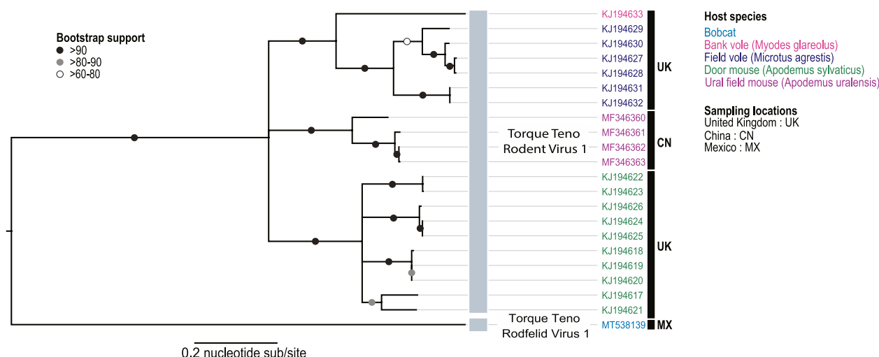
Fig. 6. Maximum-likelihood phylogeny of anelloviruses in rodent grouping 1 with one bobcat-derived anellovirus from a faecal sample. Anellovirus species are shown in grey bars. Accession numbers for the sequences are coloured based on the source/host and sampling locations are indicated with state/country codes.
