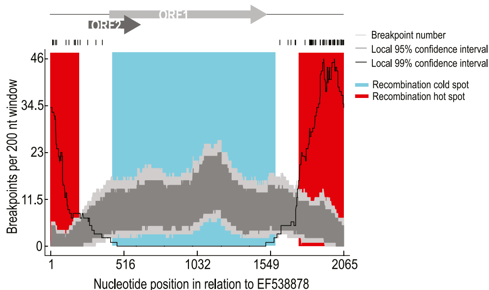
Fig. 5. Recombination hot- and cold-spots within anellovirus genomes from feline groupings 1 and 2. The black vertical lines above the figure indicate the positions of detected recombination breakpoints and the black line in the plot indicates breakpoint numbers falling within a 200-nucleotide sliding window. The red regions indicate the breakpoint hotspot and the blue region the cold-spot. The light and dark grey areas respectively indicate 99 % the 95 % confidence intervals of the expected degrees of breakpoint clustering under random recombination.
