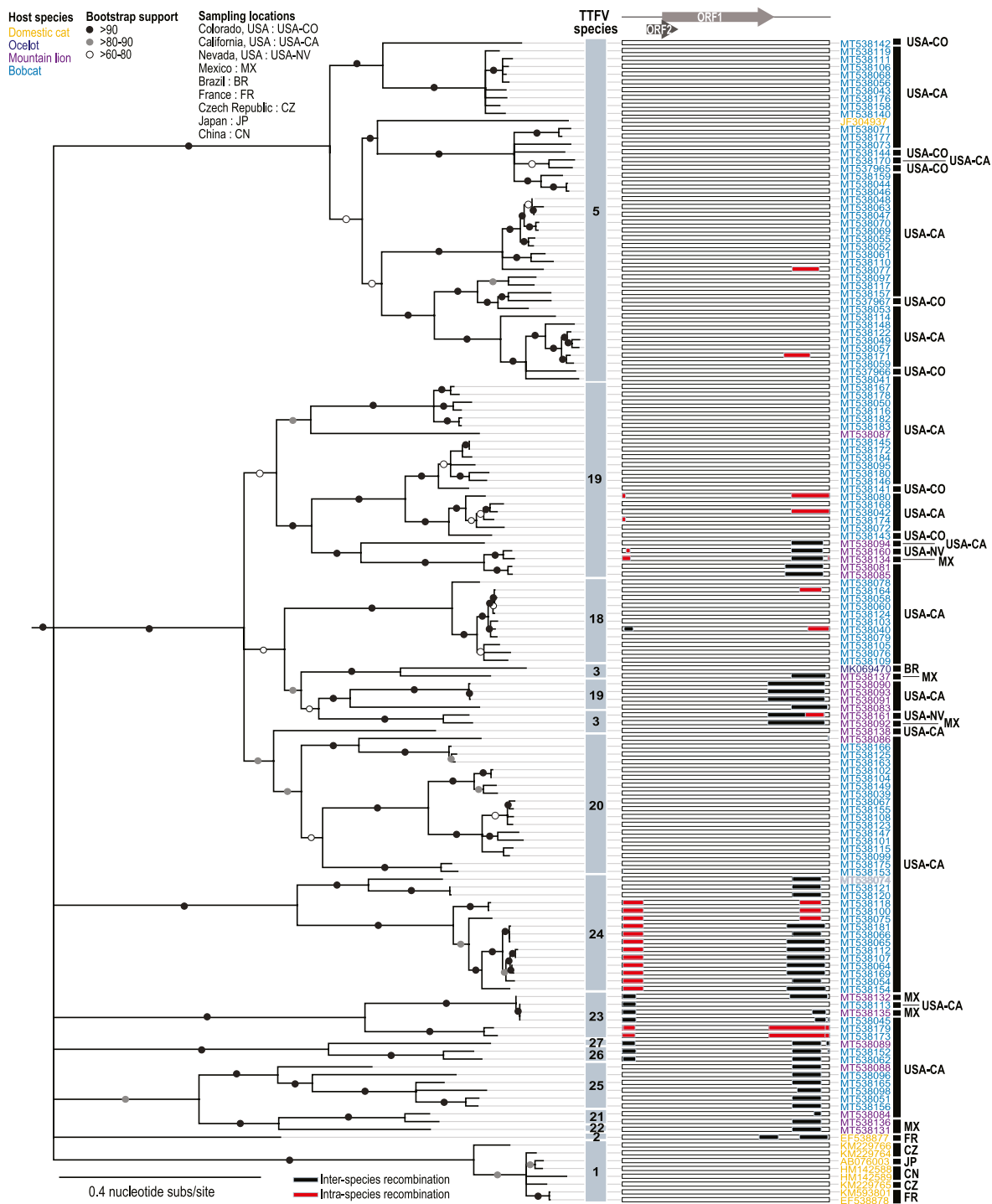
Fig. 3. Inter- and intra-species recombination events detected in bobcat and puma anelloviruses. Recombination-free maximum-likelihood phylogeny of the sequences in feline anellovirus group 1 derived from pumas, bobcats, domestic cats and an ocelot. Anellovirus species groupings are shown in the grey bar beside the tree. Recombination events are indicated in the linearized genome schematic. Accession numbers for each sequence are coloured based on the source/host and sampling location indicated by state and/or country codes.
