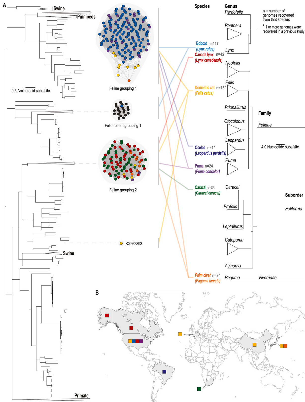
Fig. 2. Feline anelloviruses display a complex evolutionary history. A) The approximate maximum-likelihood phylogenetic tree on the left illustrates the evolutionary relationships of ORF1 proteins from all published anellovirus genomes with those recovered from felid species in this study. Protein similarity networks are shown next to the feline anellovirus clades, with each node in the network representing the ORF1 proteins from feline and palm civet derived anelloviruses. Species of sample origin are colour coded. The phylogram on the right shows the species and genus within the Feliforma Suborder; The Felidae and Viverridae families for which anelloviruses were recovered in this study, and other previously recovered anelloviruses in these groups are shown by a “*”. The numbers of isolates from each host is shown next to the general and Latin species names. B) Shows the regions from which feline and palm civet derived anelloviruses were sampled.
