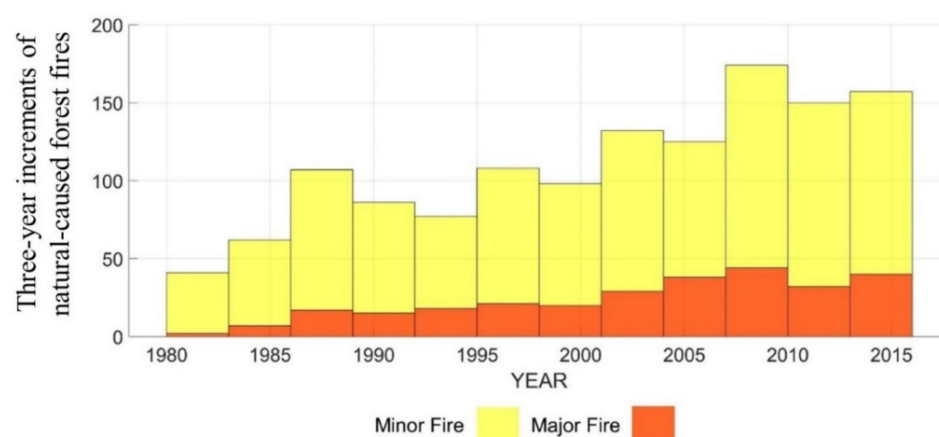
Figure 3. Three-year increments of natural-caused forest fires over the historical period (1980–2015) in western U.S. forests.
