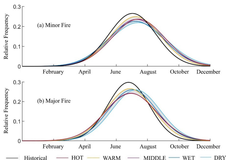
Figure 9. Monthly distribution of (a) minor and (b) major forest fires under historical (1986–2015) and future (2070–2099) climate conditions.
