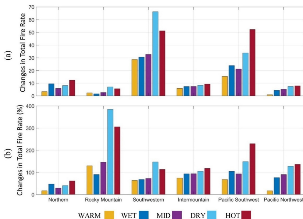
Figure 8. (a) Absolute changes in total fire rate and (b) percentage changes on total fire rate of United States Forest Service regions from historical (1986–2015) to future conditions (2070–2099).
