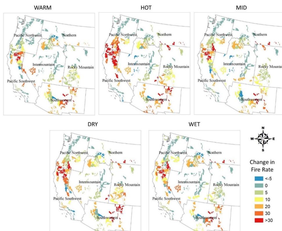
Figure 7. Changes in rate of major forest fires from historical (1986–2015) to future conditions (2070–2099) in western U.S. forests.
