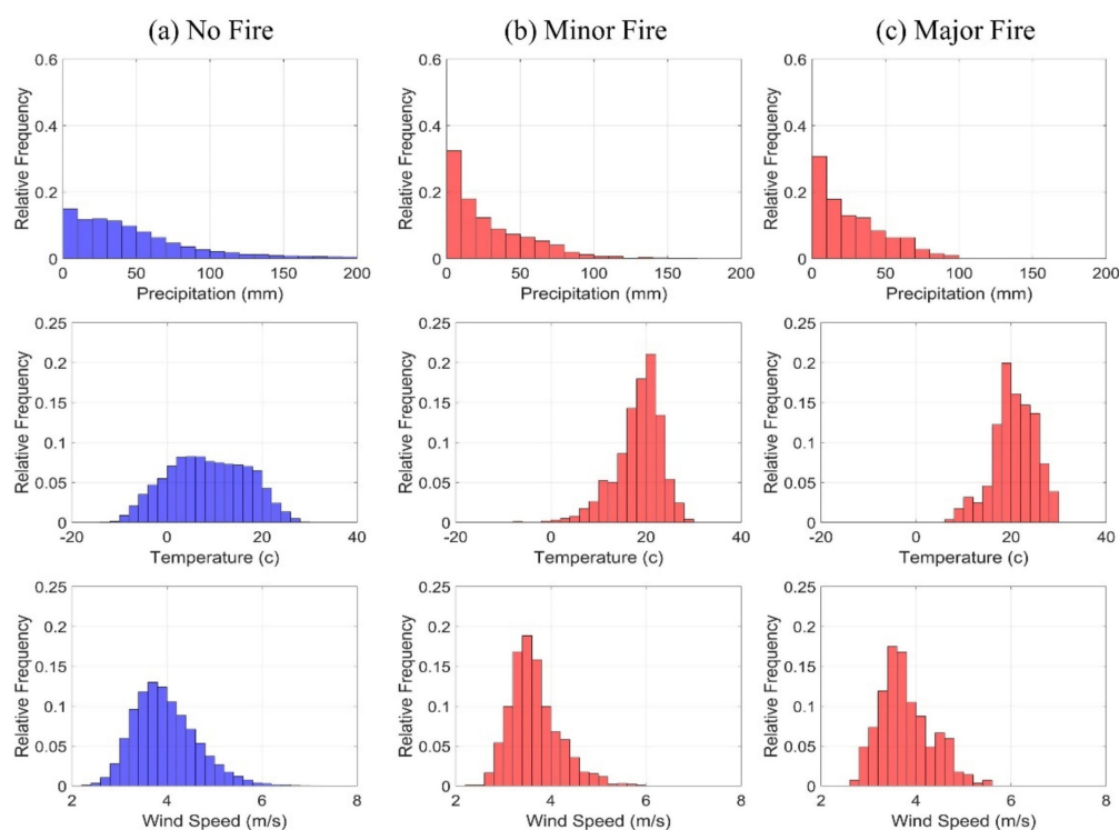
Figure 4. Relative frequency of monthly precipitation, temperature, and wind speed for months (a) without fire, (b) minor fire, and (c) major fire over the historical period (1986–2015).
