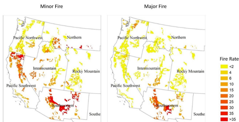
Figure 2. Total rate of minor and major forest fires in western U.S. forests over the historical period (1986–2015).
