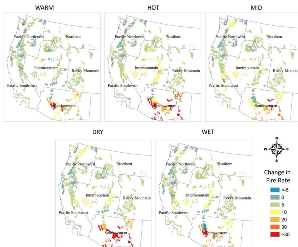
Figure 6. Changes in rate of minor forest fires from historical (1986–2015) to future conditions (2070–2099) in western U.S. forests.
