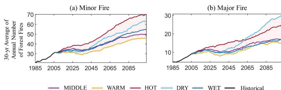
Figure 5. Changes in the rate of (a) minor fire, and (b) major fire from 1985 to 2099 under the historical and five climate scenarios.
