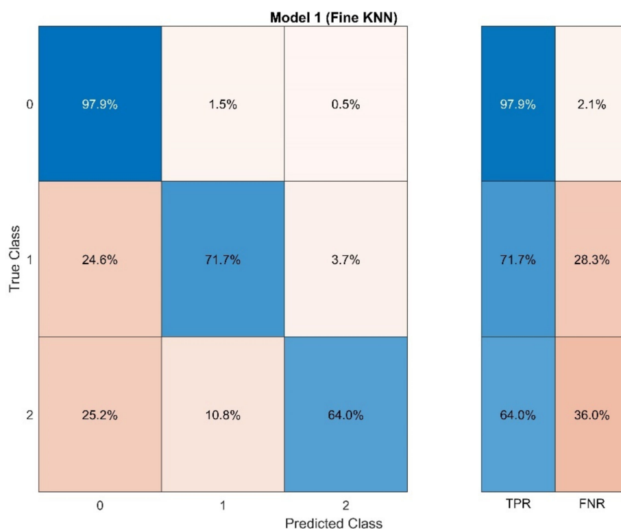
Figure 1. The confusion matrix of the Fine KNN model with 5-fold cross-validation.
