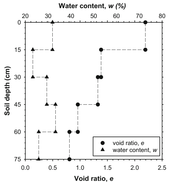
Fig. 3 Variation of water content and void ratio with soil depth for the untreated field soil
