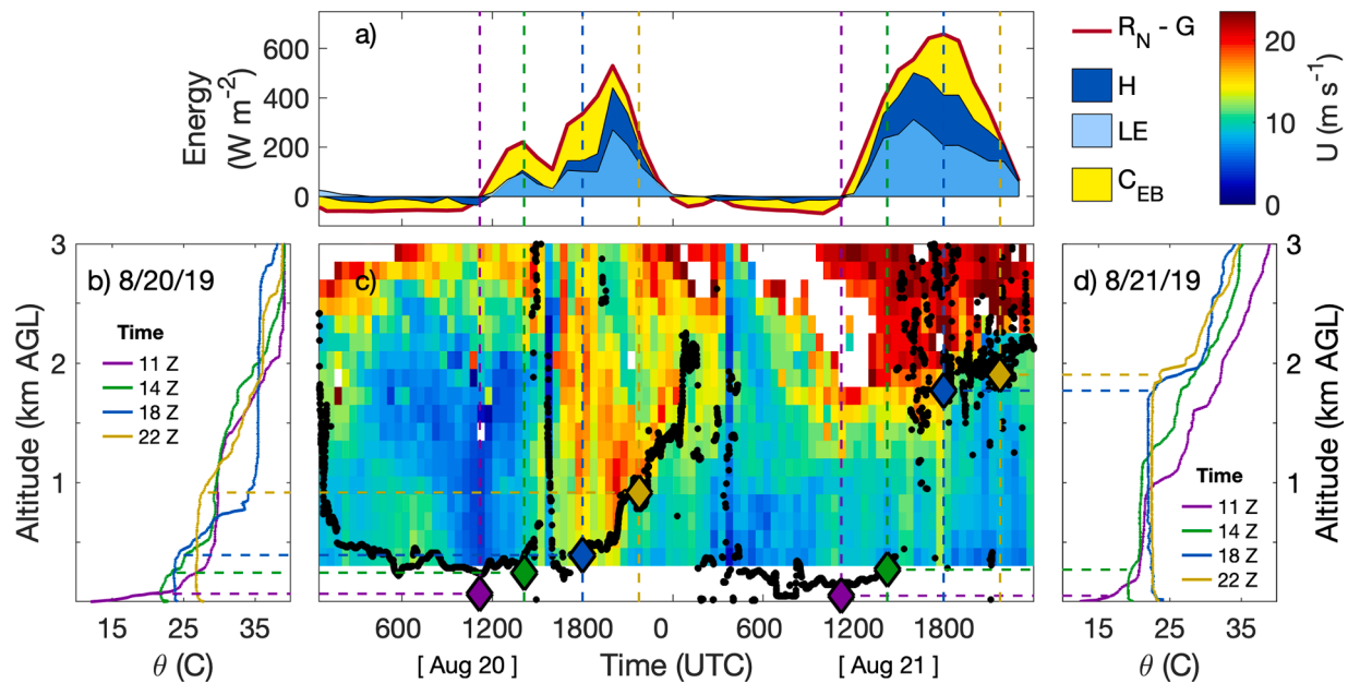
Fig. 9. (a) Cumulative (i.e., stacked) latent, sensible heat flux, and energy balance residual (LE, H, and C EB ) measured by AmeriFlux tower US-PFa at 30 m AGL with mean net radiation and ground flux (R N and G) measurements from 17 nearby eddy-covariance towers installed during the CHEESEHEAD19 field campaign; (b) and (d) daytime radiosonde profiles on August 20 and 21, 2019; and (c) winds measured by a 449 MHz radar wind profiler overlaid with Vaisala CL51 ceilometer (black circles) and radiosonde-derived (diamonds) ABL heights (NCAR/EOL In-situ Sensing Facility 2020; Butterworth et al., 2021).
