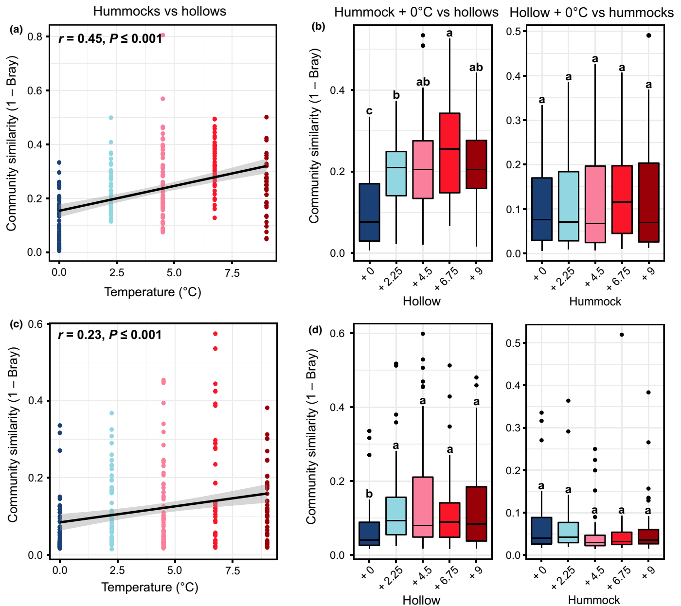
Fig. 1 Similarity (1 – Bray–Curtis dissimilarity) of bacterial (a) and fungal (c) operational taxonomic unit (OTU) composition in hummocks and hollows in each of the five temperature treatments (+ 0, + 2.25, + 4.5, + 6.75 and + 9°C) following 3 months of field incubation. Gray shading represents the 95% confidence interval. Similarity of bacterial (b) and fungal (d) OTU composition in each temperature treatment compared with the unwarmed (+ 0) hummock and unwarmed (+ 0) hollow, respectively. Different letters indicate significant differences (Tukey's honestly significant difference, P \leq 0.05 ). Boxes correspond to median (line in box), 25 th percentile (lower line) and 75 th percentile (upper line) ranges. Whiskers extend from 25 th and 75 th percentile limits to the smallest and largest values that do not exceed 1.5 \times interquartile range limit in each direction. Data beyond the end of the whiskers are plotted individually as circles.
