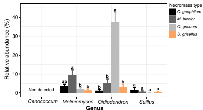
Fig. 4 The relative abundance of Cenococcum , Meliniomyces , Oidiiodendron and Suillus fungal genera depending on necromass type following 3 months of field incubation ( C. geophilum , M. bicolor , O. griseum and S. grisellus ) ( \pm SE). Different letters indicate significant differences (Tukey's honestly significant difference, P \leq 0.05 ).
