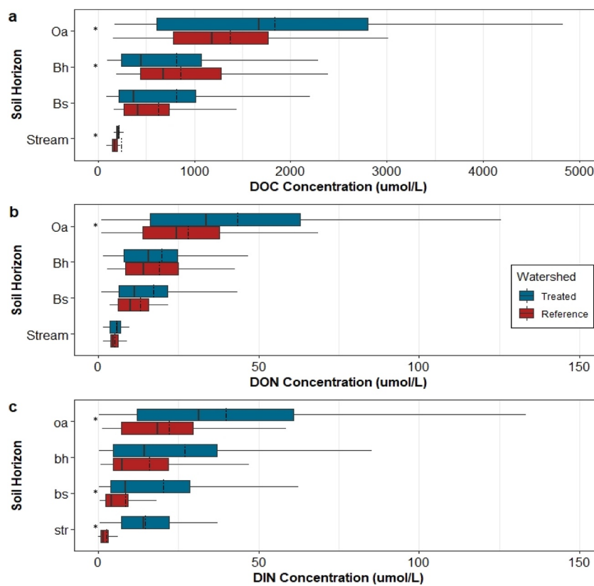
Figure 5. Box and whisker plots of (a) dissolved organic carbon (DOC), (b) dissolved organic nitrogen (DON), and (c) dissolved inorganic nitrogen (DIN) concentrations in stream and soil water, from reference and treated watersheds. Dashed lines represent median values, stream, and soil water, from reference and treated watersheds. Stars represent statistically significant differences between watersheds by Wilcoxon signed-rank test to a significance level of 0.05.
