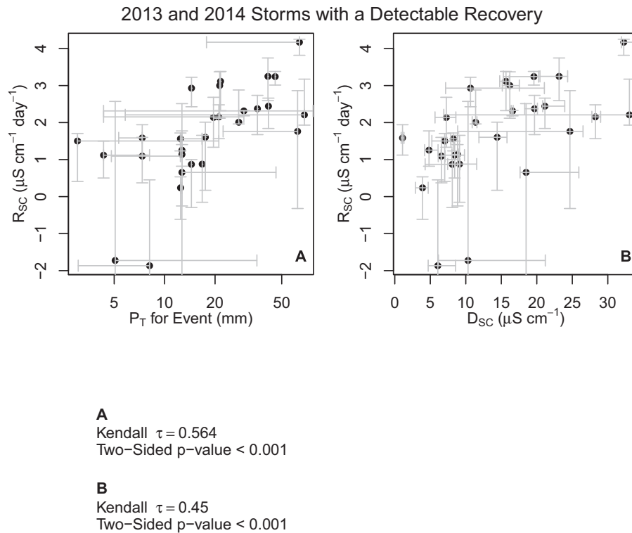
FIGURE 9. Kendall's \tau relationships for the rate of SC recovery ( R_{SC} ) and (a) precipitation intensity ( P_T ) and (b) magnitude of the dilution ( D_{SC} ). Whiskers indicate the interquartile range of the values obtained from the 10,000 iterations. An absence of whiskers indicates 100% confidence in the value across all iterations.
