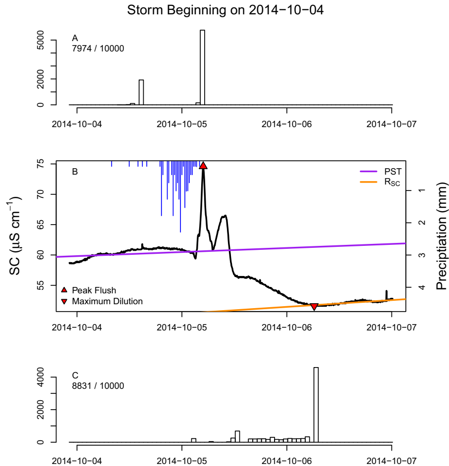
FIGURE 6. The algorithm-derived points of peak flush and maximum dilution for a precipitation event beginning on October 4, 2014 and their respective distributions. Unlike Figure 5, the earlier point for peak flush is chosen more frequently by the algorithm because the first has a greater SC. In this way, the algorithm retains the truest representation of a flush despite later options being available. (a) The distributions of algorithm derived peak flush values (number of times a peak flush was detected/number of times the precipitation event was detected). (b) The median of the extracted peak flush and maximum dilution values from each of the algorithm's iterations. These points overlay the SC data surrounding the precipitation event. The PST and rate of SC recovery ( R_{SC} ) are also displayed with estimated intercepts for appropriate visual representation. (c) The distribution of algorithm derived maximum dilution values (number of times a maximum dilution was detected/number of times the precipitation event was detected).
