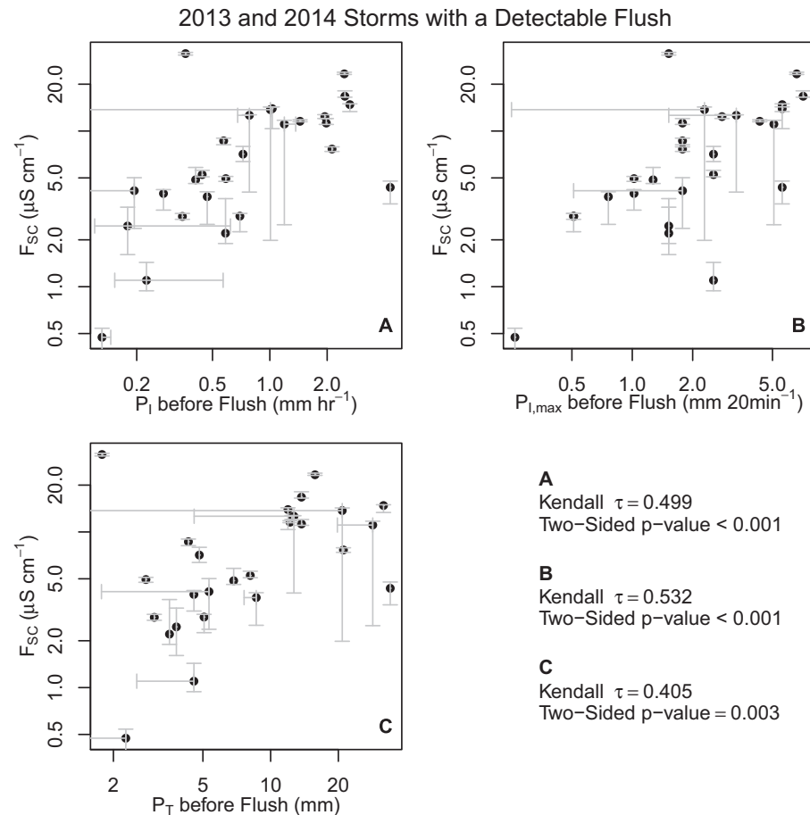
FIGURE 7. Kendall's \tau relationships for the magnitude of peak flush ( F_{SC} ) and A) precipitation intensity ( P_I ), B) maximum precipitation intensity ( P_{I,max} ), and C) total precipitation ( P_T ). Whiskers indicate the interquartile range of the values obtained from the 10,000 iterations. An absence of whiskers indicates 100% confidence in the value across all iterations.
