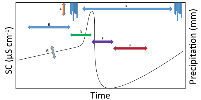
FIGURE 4. A visual representation of the parameter ranges for the Monte Carlo calculations. Parameter description: (A) the minimum amount of precipitation for an event to be considered for analysis, (B) both the time between individual precipitation measurements that separated unique events, and the range of time to define the PST, (D) the amount of time for a flushing response to be found after the storm began, (E) the amount of time for a dilution response to be found after the flush occurred, or after 6 h prior to the end of the storm's precipitation if no substantial flush was present, (F) the amount of time in which the slope of the rate of SC recovery was calculated after the dilution, and (G) the number of standard deviations above or below the PST line that a peak flush or maximum dilution must have exceeded in order to be declared substantial enough for analysis.
