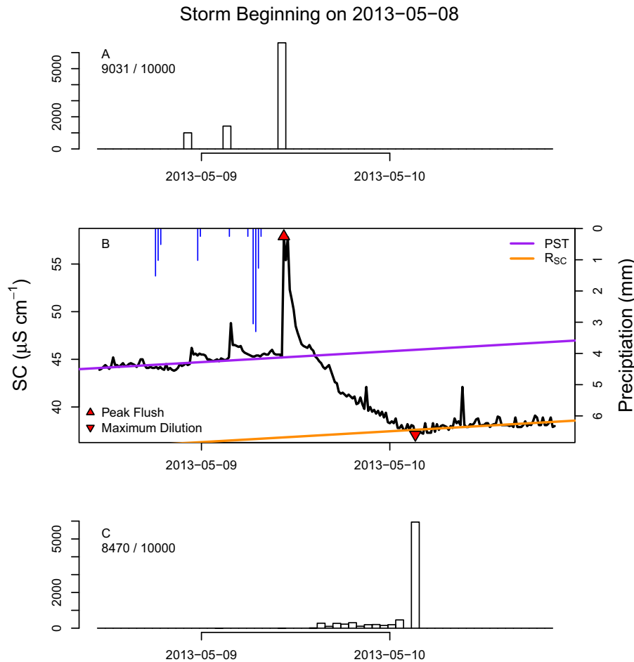
FIGURE 5. The algorithm-derived points of peak flush and maximum dilution for a precipitation event beginning on May 8, 2013 and their respective distributions. Of note are the three points in which a peak flush was found across iterations, due to the variable range of Parameter D, and the increasing SC values of those points occurring in time. In this way, the algorithm seeks the truest representation of a flush over time. (a) The distributions of algorithm derived peak flush values (number of times a peak flush was detected/number of times the precipitation event was detected). (b) The median of the extracted peak flush and maximum dilution values from each of the algorithm's iterations. These points overlay the SC data surrounding the precipitation event. The PST and rate of SC recovery ( R_{SC} ) are also displayed with estimated intercepts for appropriate visual representation. (c) The distribution of algorithm derived maximum dilution values (number of times a maximum dilution was detected/number of times the precipitation event was detected).
