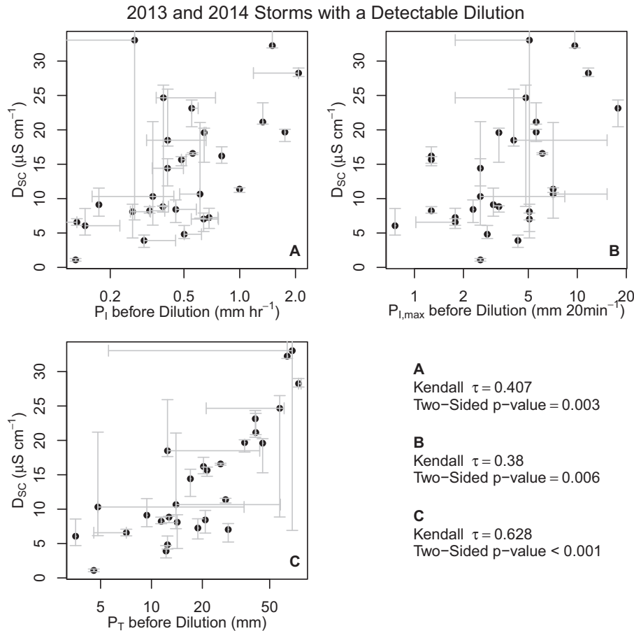
FIGURE 8. Kendall's \tau relationships for the magnitude of maximum dilution ( D_{SC} ) and (a) precipitation intensity ( P_I ), (b) maximum precipitation intensity ( P_{I,max} ), and (c) total precipitation ( P_T ). Whiskers indicate the interquartile range of the values obtained from the 10,000 iterations. An absence of whiskers indicates 100% confidence in the value across all iterations.
