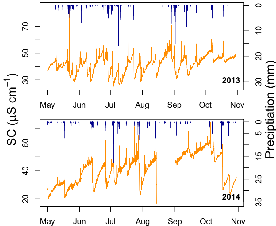
FIGURE 3. The full record of SC and precipitation data for the months we analyzed in both 2013 and 2014.
