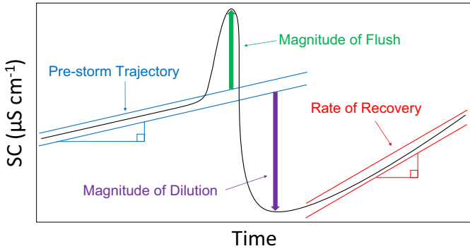
FIGURE 1. A conceptual model of the specific conductivity (SC) patterns that streamwater takes during and after a precipitation event. Highlighted are the aspects that we use to characterize the watershed response to individual precipitation events: the flush, dilution, and rate of SC recovery. Also shown is the pre-storm trajectory, or the course of streamwater SC prior to the influence of a precipitation event, which is used to quantify both the magnitude of the flush and the magnitude of the dilution.
