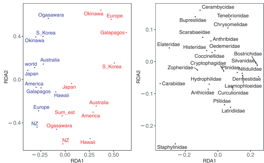
FIGURE 6 Results of RDA ordination on numbers of species per family. (a) location of each region in space defined by first two RDA axes; native assemblages in blue; non-native assemblages in red. (b) Loadings for each family
