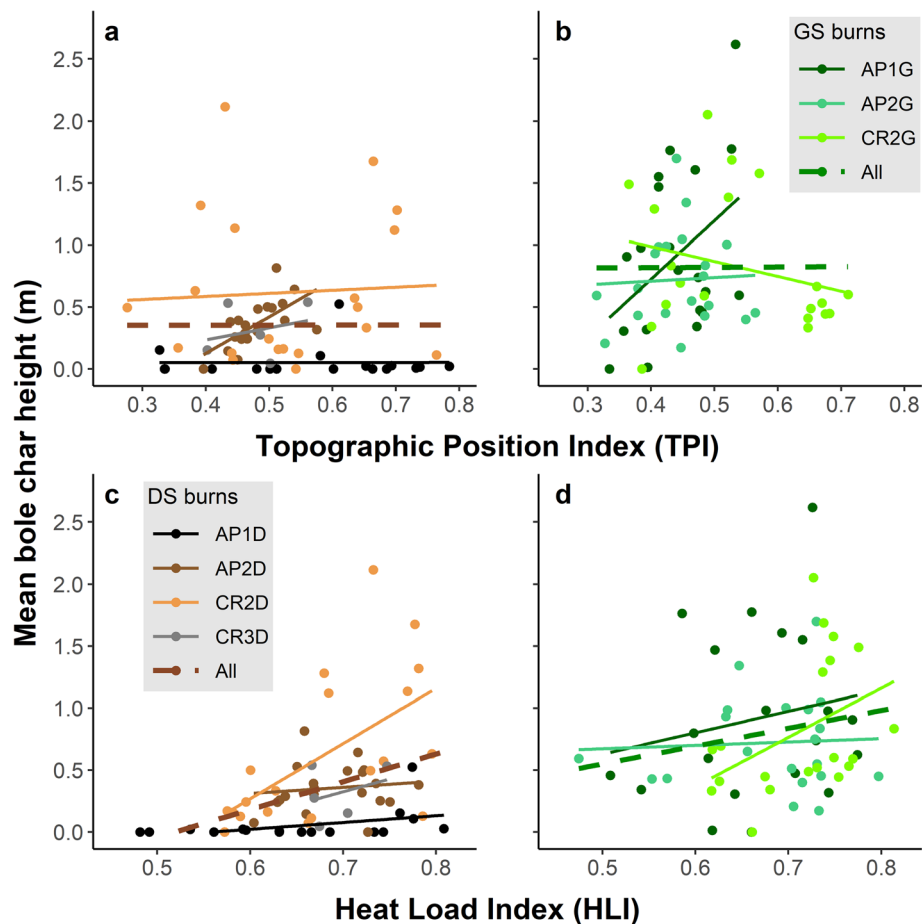
Fig. 8 Scatterplots with linear regressions of mean bole char height (y-axis; m) vs. landscape indices Topographic Position Index (TPI) and Heat Load Index (HLI) (x-axis) by burn treatment (columns) and index (rows) for all plots in each unit (series). Top row, left column shows mean bole char height vs. TPI for dormant season burns (a), top row, right column shows mean bole char height vs. TPI for growing season burns (b), bottom row, left column shows mean bole char height vs. HLI for dormant season burns (c), and bottom row, right column shows mean bole char height vs. HLI for growing season burns (d)
