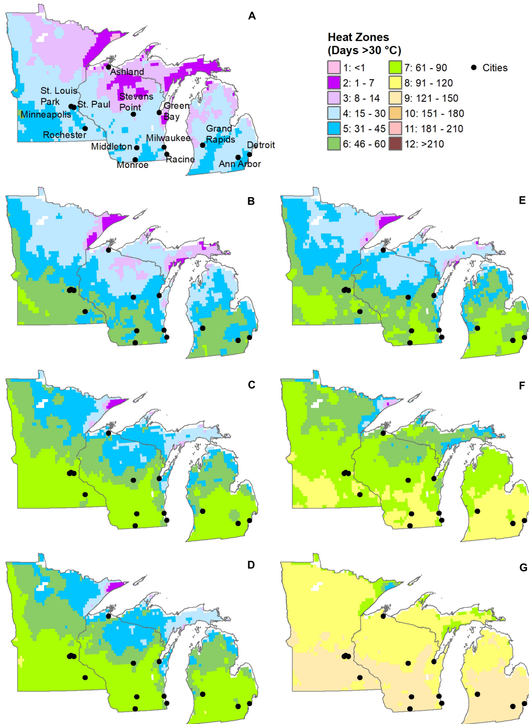
FIGURE 4 | AHS Heat Zones under (A) current climate (1980–2009) and future climates under a low emissions pathway (B–D, 2010–2039, 2040–2069, 2070–2099) or high emissions pathway (E–G, 2010–2039, 2040–2069, 2070–2099). Data from Matthews et al. (2018).
