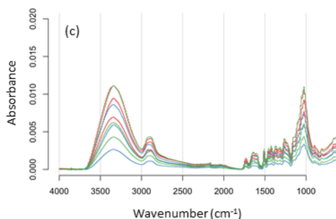
Figure 3. Representative FT-IR spectra in the range 4000–650 \text{cm}^{-1} for Alaska yellow cedar samples according to durability classifications established by exposure to (a) G. trabeum , (b) R. placenta , and (c) R. flaviges . Green = highly resistant, blue = resistant, red = non-resistant.
