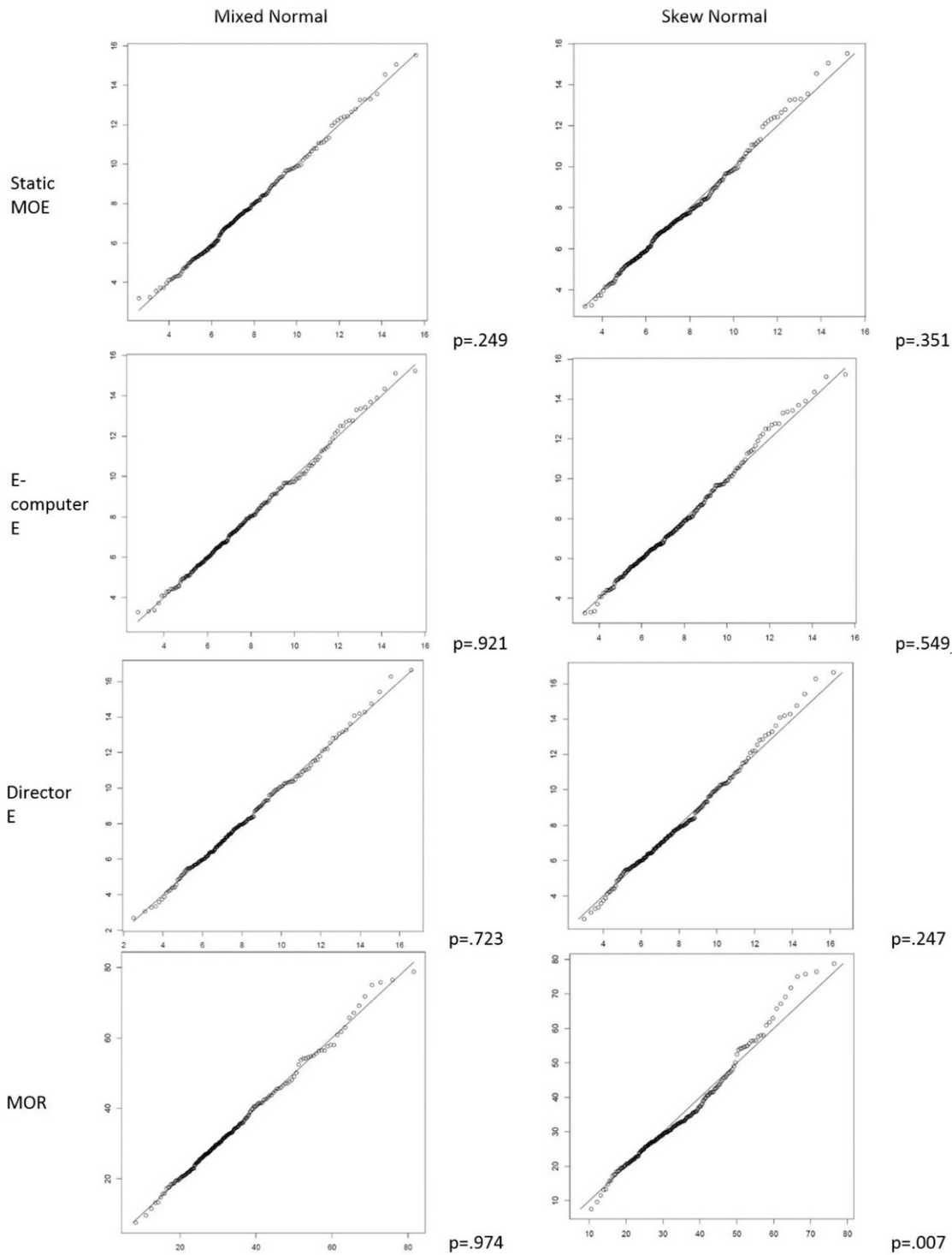
Figure 3. Probability plots for skew normal and mixed normal distributional fits to bending properties in red pine. For each plot, X and Y axes are “ordered expected values” and “ordered observed values,” respectively. The p -values are from Cramér–von Mises simulation tests.
