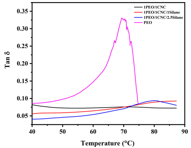
Figure 8. Tan \delta curves as a function of temperature for PEO, untreated CNC incorporated PEO, (1:1) silane treated and (1:2.5) silane treated CNC incorporated samples.
