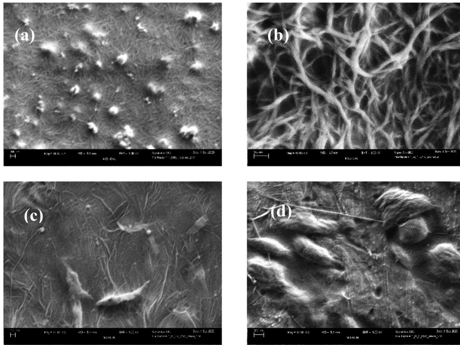
Figure 3. SEM images of PEO-CNC composite films: (a) 1PEO/1CNC, (b) 1PEO/1CNC/1Silane, (c) 1PEO/1CNC/2.5Silane and (d) 1PEO/1CNC/5Silane samples.
