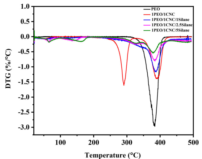
Figure 5. Derivative thermogravimetric (DTG) curves of PEO, untreated CNC incorporated PEO, (1:1) silane treated, (1:2.5) silane treated and (1:5) silane treated CNC incorporated samples.
