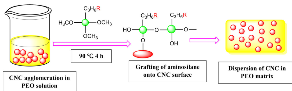
Figure 1. Reaction mechanism of silane grafting onto CNC surface.
