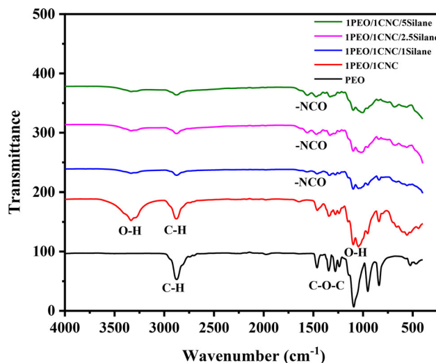
Figure 2. Transmission spectra of PEO, untreated CNC incorporated PEO, (1:1) silane treated, (1:2.5) silane treated and (1:5) silane treated CNC incorporated samples measured using FTIR.
