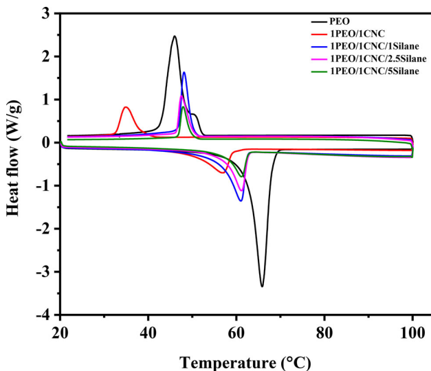
Figure 6. DSC thermograms of PEO, untreated CNC incorporated PEO, (1:1) silane treated, (1:2.5) silane treated and (1:5) silane treated CNC incorporated samples.
