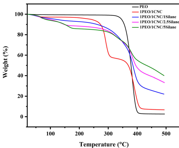
Figure 4. TGA thermogram of PEO, untreated CNC incorporated PEO, (1:1) silane treated, (1:2.5) silane treated and (1:5) silane treated CNC incorporated samples.
