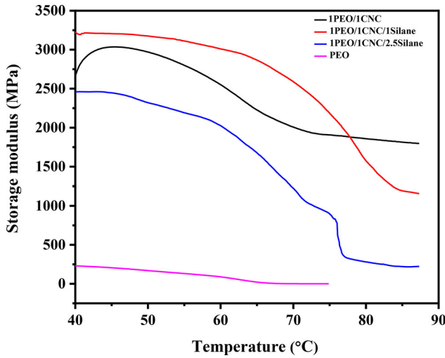
Figure 7. Representative curve of storage modulus as a function of temperature of PEO, untreated CNC incorporated PEO, (1:1) silane treated and (1:2.5) silane treated CNC incorporated samples.
