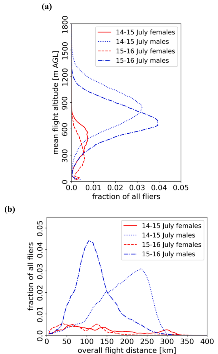
Fig. 11. Simulated SBW (a) mean flight altitudes and (b) flight distances for 14,15 July and 15,16 July 2013.
