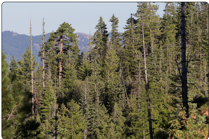
Figure 3. View near Tronsen Ridge (in the background), 2013, Okanogan-Wenatchee National Forest, Washington. Only a handful of trees in this scene were present 125 to 150 years ago. The largest ponderosa pines are 300 to 400 years old, developing under a frequent fire regime. Most other trees are fire-intolerant grand fir and Douglas fir that established over the period of livestock grazing and fire exclusion. A few dwarf mistletoe infested younger western larch are dead in this scene owing to extreme intertree competition for soil moisture and nutrients, and mistletoe infection severity.
