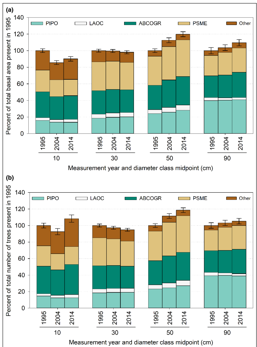
Figure 1. Species abundance has changed in mixed-conifer forests in recent decades. Estimates of (a) basal area per hectare (BAH) and (b) trees per hectare (TPH) on public lands in eastern Oregon and Washington were compiled from national and regional forest inventories. For each diameter class, bars from left to right represent estimates for midpoint inventory years 1995 (1990–1999), 2004 (2000–2007), and 2014 (2010–2017). Species include the fire-tolerant and shade-intolerant ponderosa pine ( Pinus ponderosa , PIPO) and western larch ( Larix occidentalis , LAOC); the shade-tolerant white fir ( Abies concolor ) or grand fir ( Abies grandis ) (together, ABCOGR) and Douglas fir ( Pseudotsuga menziesii , PSME); and all other tree species combined (Other). Species proportions in 2004 and 2014 are relative to the BAH (above) and TPH totals (below) in 1995, for each diameter class. Diameter class midpoints are (left to right) 10 cm (range 2.5–20 cm), 30 cm (range 20–40 cm), 50 cm (range 40–60 cm), and 90 cm (range 60–120 cm). Results show overall increases in BAH and TPH for tree diameters >40 cm, with ABCOGR and PSME increasing more than PIPO, and LAOC generally declining. Error bars represent the standard error of the mean estimate. (a) The proportions of total BAH in the 10-cm, 30-cm, 50-cm, and 90-cm midpoint classes in 2014 were 16.9%, 35.1%, 27.5%, and 20.6%, respectively. (b) The proportions of total TPH in the 10-cm, 30-cm, 50-cm, and 90-cm midpoint classes in 2014 were 79.9%, 14.5%, 4.2%, and 1.4%, respectively. Note that the largest increases in BAH and TPH occurred in the 50-cm class.
