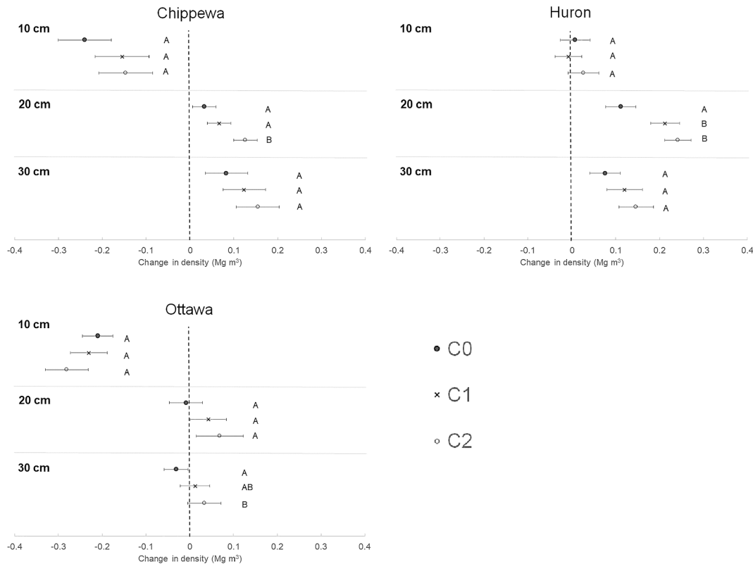
Fig. 4. Change in bulk density by site, treatment, and depth increment. Negative values indicate lower bulk density than pretreatment; positive values indicate higher bulk density than pretreatment. Error bars are 90% confidence limits. Bars which do not overlap the zero line are significantly different from zero.
