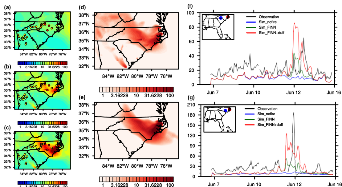
Figure 12. The PM 2.5 distribution and time series during the 2008 Evans Road Fire. (a–c) PM 2.5 daily mean surface concentration (μg m -3 ) on 12 June 2008 simulated in (a) sim_nofire, (b) sim_FINN, and (c) sim_FINN+duff runs. (d–e) The PM 2.5 daily surface concentration differences (μg m -3 ) between (d) sim_FINN and sim_nofire and between (e) sim_FINN+duff and sim_FINN on 12 June 2008. (f–g) The comparison of the time series of hourly surface PM 2.5 concentrations (μg m -3 ) between the observation and simulations from 7 to 14 June 2008 in (f) Mecklenburg County, North Carolina, and (g) Cumberland County, North Carolina.
