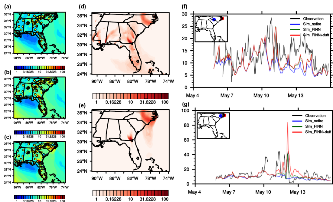
Figure 13. The PM 2.5 distribution and time series during the 2011 Pains Bay Fire. (a–c) PM 2.5 daily mean surface concentration (μg m -3 ) on 12 May 2011 simulated in (a) sim_nofire, (b) sim_FINN, and (c) sim_FINN+duff runs. (d–e) The PM 2.5 daily surface concentration differences (μg m -3 ) between (d) sim_FINN and sim_nofire and between (e) sim_FINN+duff and sim_FINN on 12 May 2008. (f–g) The comparison of the time series of hourly surface PM 2.5 concentrations (μg m -3 ) between the observation and simulations from 6 to 15 May 2011 in (f) Mecklenburg County, North Carolina, and (g) Wayne County, North Carolina.
