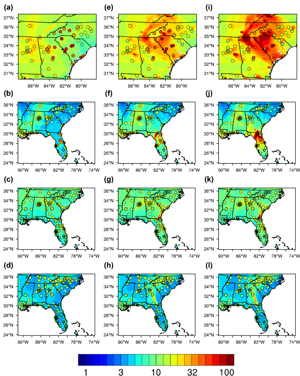
Figure 6. The mean surface concentration of simulated and observed \text{PM}_{2.5} ( \mu\text{g m}^{-3} ) on representative days. (a) App16 (15 November 2016), (b) Oke07 (10 May 2007), (c) Oke11 (8 May 2011), and (d) Oke17 (29 April 2017) for sim_nofire . Panels (e)–(h) are the corresponding fire cases for sim_FINN , and panels (i)–(l) are the corresponding fire cases for sim_FINN+duff . The color scatters represent the observed daily mean \text{PM}_{2.5} concentrations.
