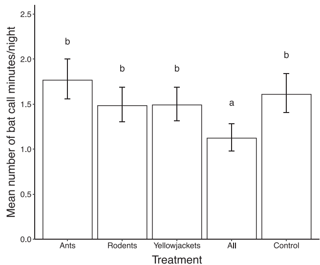
FIGURE 3 Mean number of minutes in a night containing Hawaiian hoary bat echolocations in all 5 treatment types at Pōhakuloa Training Area, Hawai‘i, USA, November 2016–January 2018. Estimated marginal means and 95% confidence intervals are based on a negative binomial generalized linear regression model and are back-transformed from the log scale to the response scale. We computed pairwise comparisons between the levels of treatment and post hoc Tukey adjusted P -values on the log scale with a family-wise error rate of 0.95. Letters in common are not significantly different. The all treatment represents ant + rodent + yellowjacket reduction
