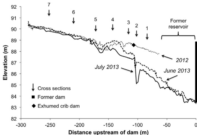
Fig. 11. Longitudinal profile for the upstream reach. Distances are shown as negative numbers indicating distance upstream of the former dam. The upper line is pre-dam removal. The middle line is post-removal but pre-flood. The lower line is post-flood. Numbers and arrows refer to sampled cross sections. Dam height is ~88.8 m.
