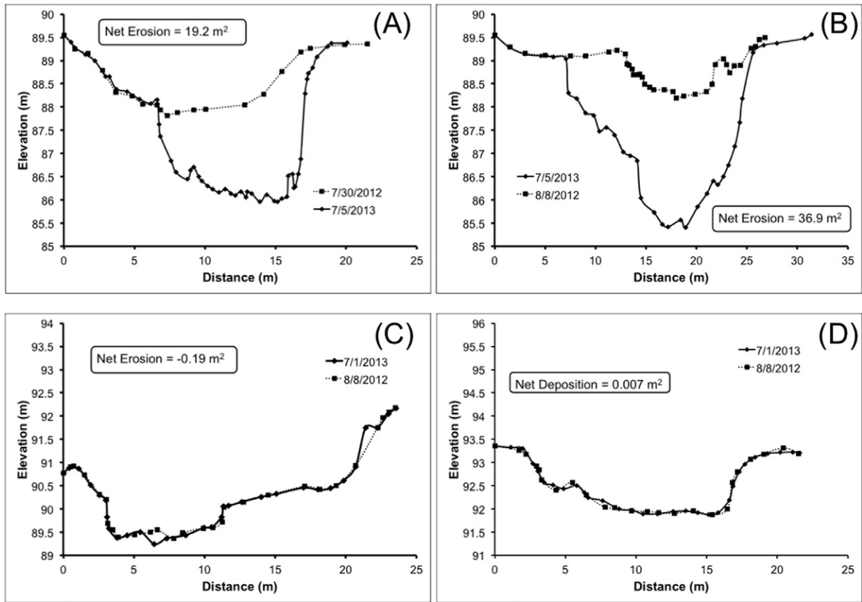
Fig. 13. Changes in representative cross sections upstream of the former dam. Cross sections 1 (A) and 2 (B) are below the exhumed crib dam. Cross sections 6 (C) and 7 (D) are at the beginning of the reach and are well above the crib dam (see Figs. 3 and 12 for location of cross sections).
