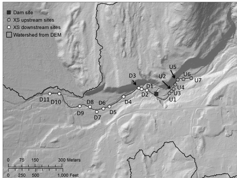
Fig. 3. Shaded DEM of Amethyst Brook, MA with location of Pelham dam and sampled cross sections along the study reach.
