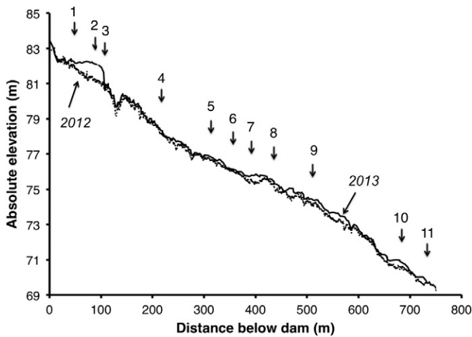
Fig. 15. Pre-removal (2012) and post-removal (2013) bed elevations along the longitudinal profile for the downstream reach.
