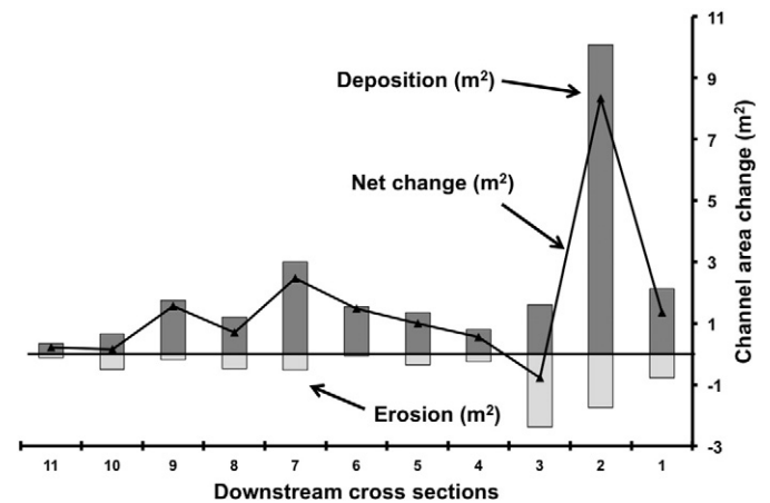
Fig. 14. Post-removal net deposition downstream of the former dam for channel cross sections. See Figs. 3 and 11 for location of cross sections.
