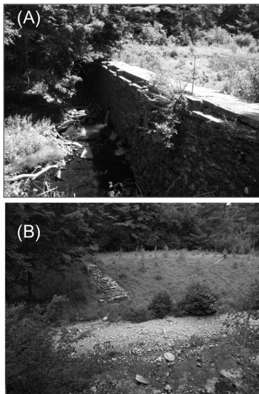
Fig. 1. View of Pelham dam pre- and post-removal. View in (A) is from below the dam on river left looking upstream. Note the level of sediment fill up to the dam crest. View in (B) is from river left to river right. Note the reconnected sediment flux through the former dam site.
