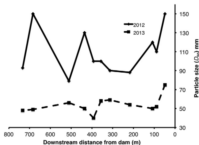
Fig. 4. Median bed particle size downstream of dam. Solid line is pre-dam and dashed line is post-dam.
