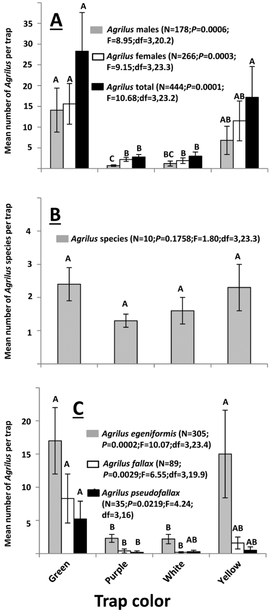
Figure 6. Mean number of A) Agrilus males, females and total; B) Agrilus species; and C) the three most common Agrilus species captured on different colored sticky traps suspended from branches of honeylocust trees at Michigan State University Tree Research Center, Ingham County, MI (Lat 42.67 N, Long -84.47) from 31 May–27 July 2011. Means within each Agrilus group, sex and species followed by a different letter are significantly different at the P < 0.05 level (Bonferroni multiple comparison test).
