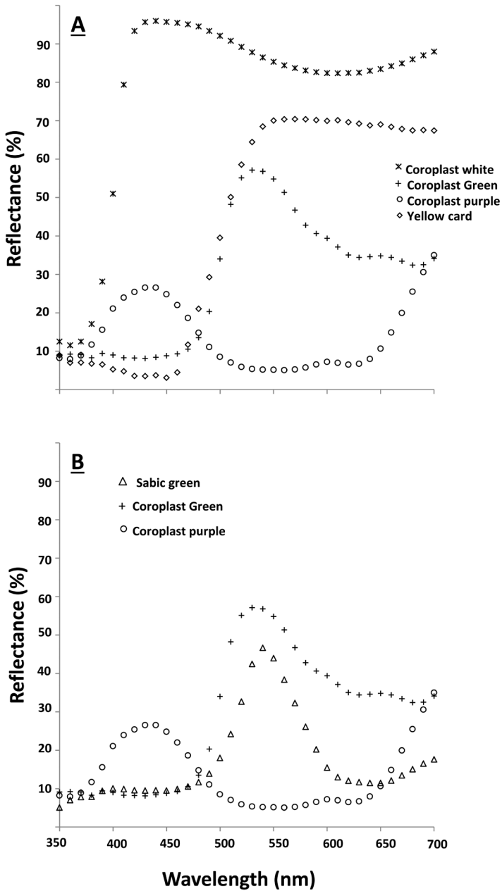
Figure 2. Reflectance spectra of A) Coroplast™ green, yellow sticky card, Coroplast™ purple, and Coroplast™ white sticky traps tested in the 2009 Agrilus subcinctus study and the 2011 hybrid poplar and honeylocust studies; and B) Coroplast™ green, Coroplast™ purple, and Sabic green tested in 2012.
