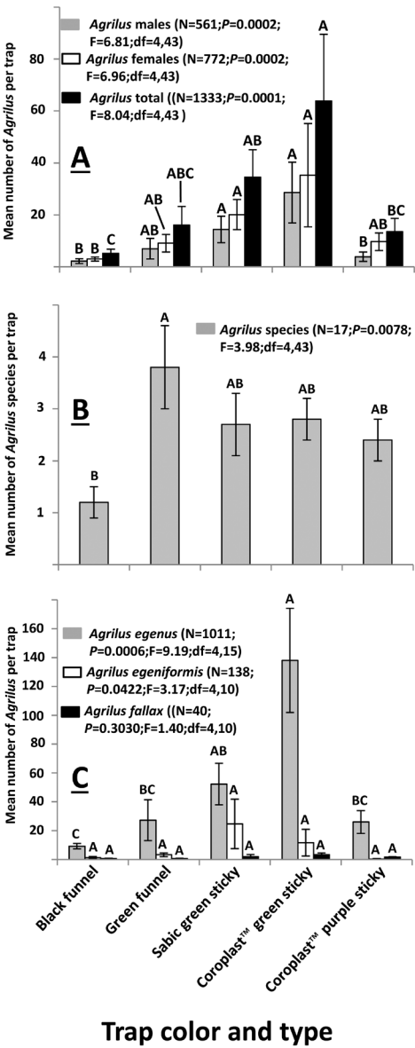
Figure 8. Mean number of A) Agrilus males, females and total; B) Agrilus species captured on traps placed around the edge of black locust, honeylocust, and English oak/white oak plantings combined; and C) A. egenus captured on traps around the black locust planting, and A. fallax and A. egeniformis captured around the honeylocust planting. Traps were suspended from rebar poles at Michigan State University Tree Research Center, Ingham County, MI (Lat 42.67 N, Long -84.47) from 8 June–24 July 2012. Means within each Agrilus group, sex and species followed by a different letter are significantly different at the P < 0.05 level (Bonferroni multiple comparison test).
