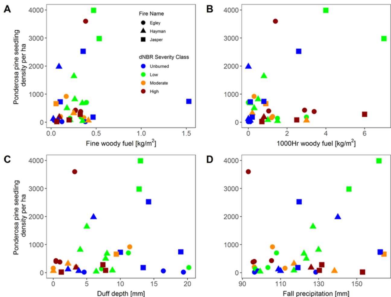
Figure 1. Predictors from best-fit non-parametric multiplicative regression (NPMR) model (see Table 2) for ponderosa pine seedling density across burn severity classes following three large wildfires. Predictors are (A) fine downed woody fuel load, (B) 1000-hr downed woody fuel load, (C) duff depth, and (D) fall precipitation.
