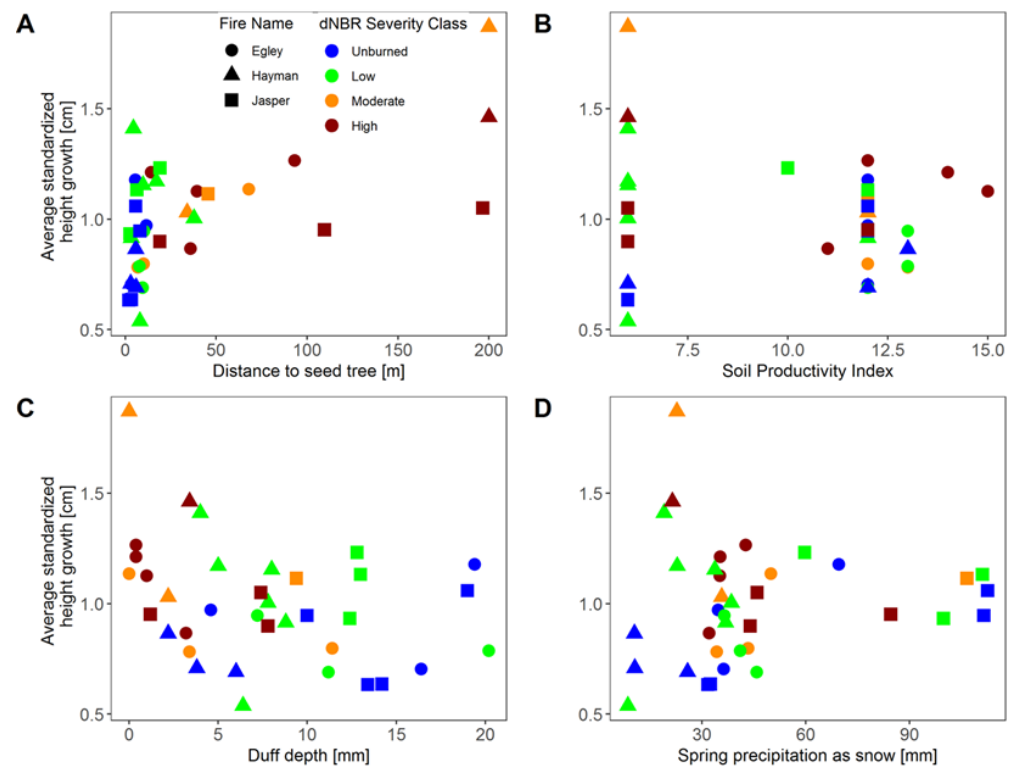
Figure 4. Predictors from best-fit non-parametric multiplicative regression (NPMR) model (see Table 2) for average height growth of ponderosa pine seedlings across a burn severity gradient following three large wildfires. Predictor variables are (A) distance to seed tree, (B) soil Productivity Index, (C) duff depth, and (D) spring precipitation as snow.
