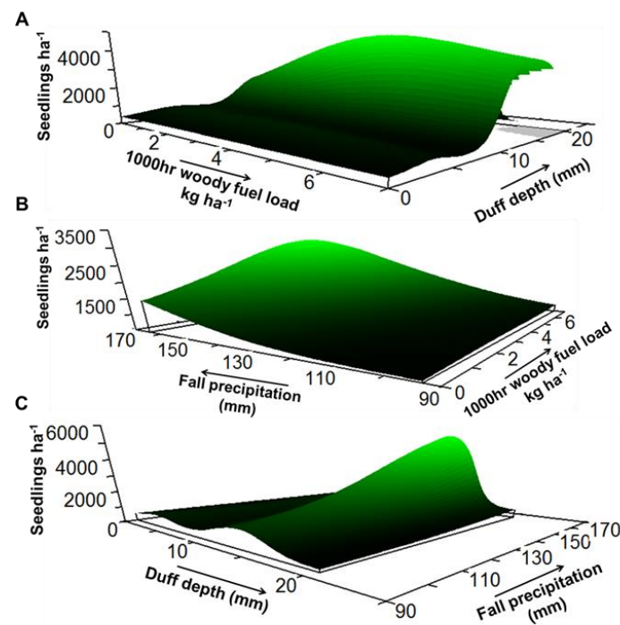
Figure 3. Ponderosa pine seedling density was impacted by 1000 h woody fuel load, which interacted with (A) duff depth, (B) fall precipitation, and by the interaction of (C) duff depth and fall precipitation. Grey areas indicate where the model lacked enough information to reliably predict the response. Note that y -axis ranges and orientation of x -axis may vary among panels.
