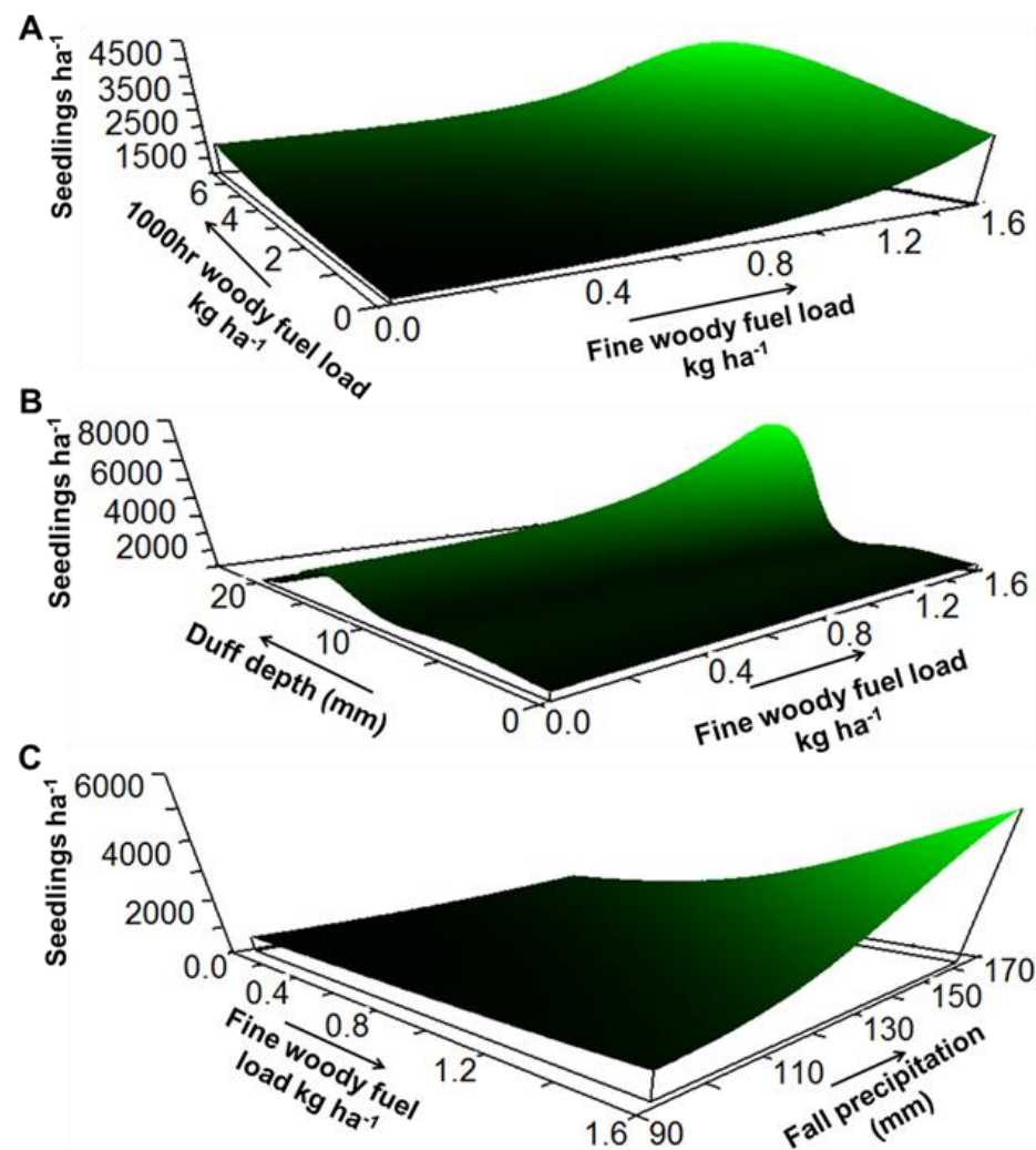
Figure 2. Ponderosa pine seedling density was impacted by fine woody fuel load, which interacted with (A) 1000 h woody fuel load, (B) duff depth, and (C) fall precipitation. Note that y-axis ranges and orientation of x-axis may vary among panels.
