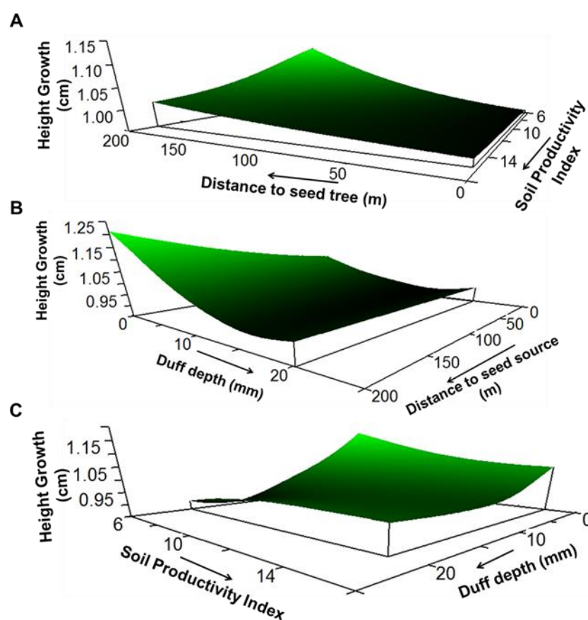
Figure 5. Average annual standardized height growth of natural ponderosa pine regeneration was impacted by distance to nearest seed source and (A) soil productivity index (soil PI) and (B) duff depth, as well as (C) soil PI and duff depth. Note that y-axis ranges and orientation of x-axis may vary among panels.
