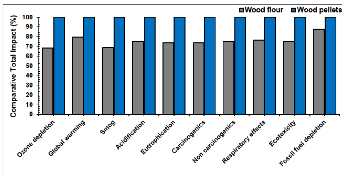
Figure 5 Comparative impact assessments for one truckload of wood flour and pellets.
