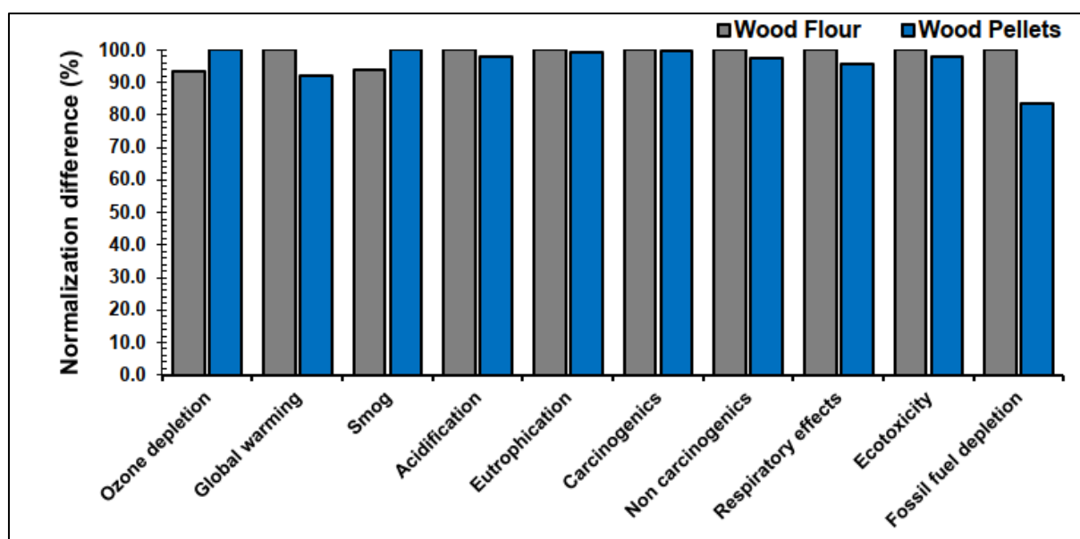
Figure 7 Comparative normalization based on the LHV of the wood feedstocks.
