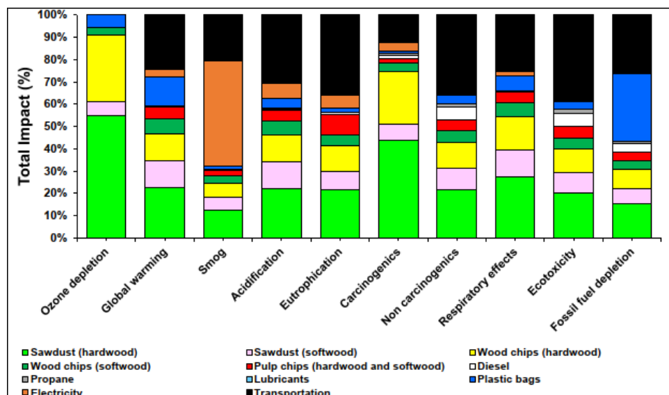
Figure 2 Impact assessment graph showing the relative contribution of the inputs for one tonne of wood flour.
