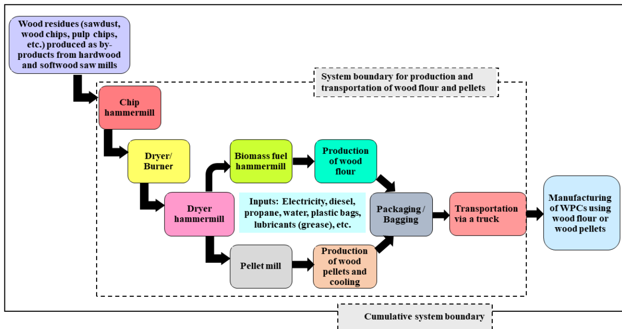
Figure 1 Unit processes and system boundary of the study.
