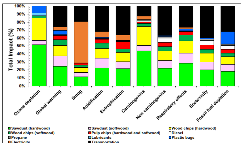
Figure 3 Impact assessment graph showing the relative contribution of the inputs for one tonne of wood pellets.
