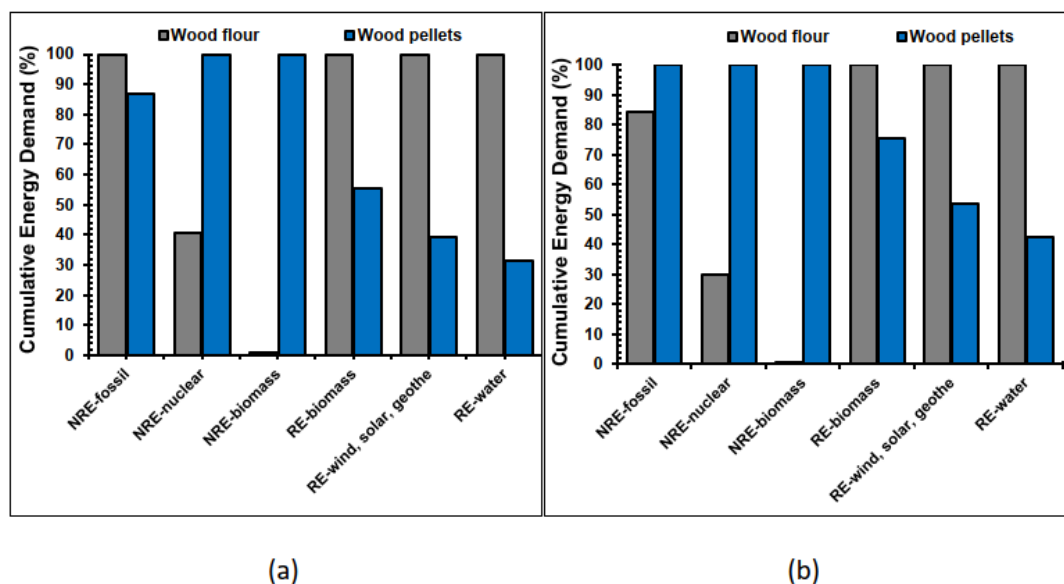
Figure 8 Comparative CED diagram for wood flour and pellets as functional unit of (a) one tonne and (b) one truckload.
