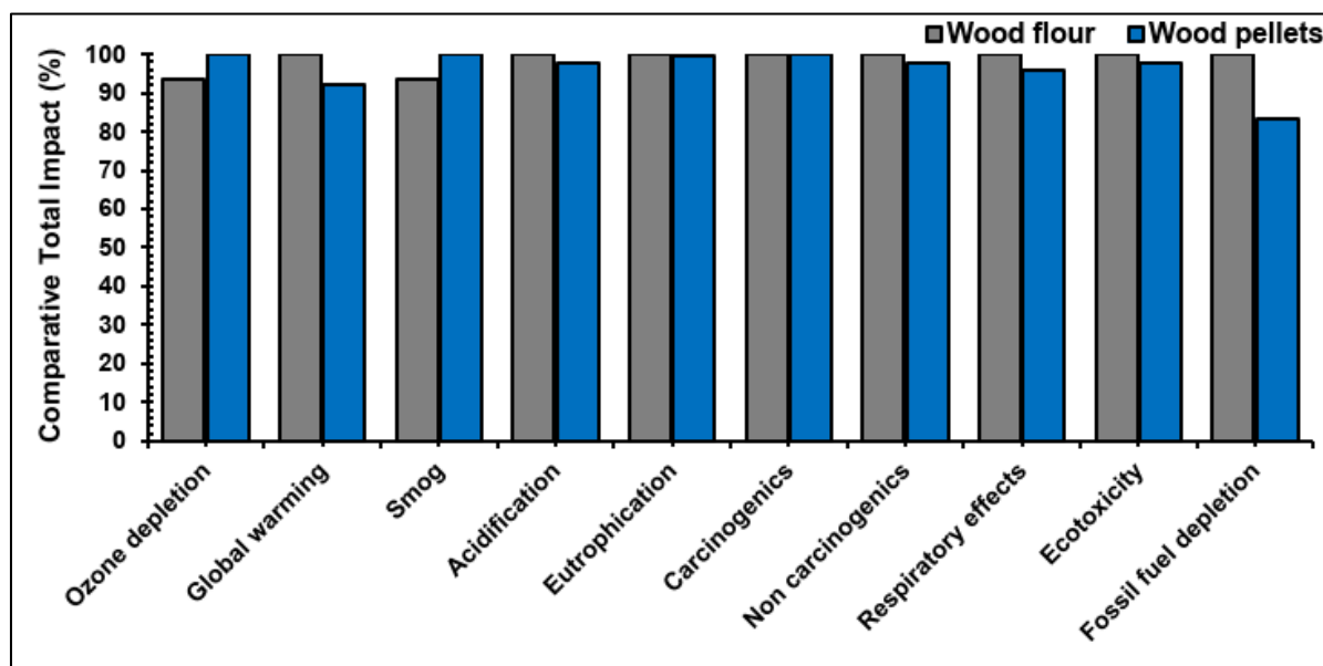
Figure 4 Comparative impact assessments for one tonne of wood flour and pellets.
