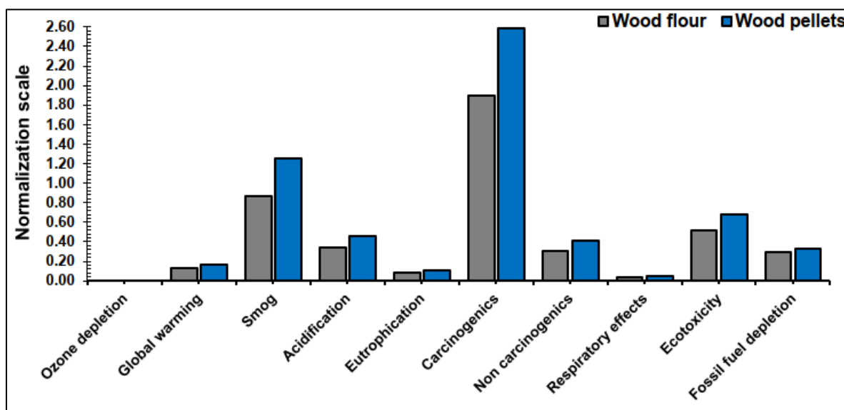
Figure 6 Comparative normalization based on SimaPro normalization factors.
