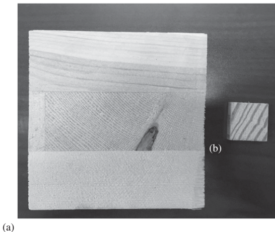
Figure 1. Comparison between cross-laminated timber (CLT) and standard test samples: (a) CLT test block face with dimensions of 10 cm \times 10 cm \times 2.5 cm (length \times width \times thickness); (b) American Wood Protection Association (AWPA) E1-17 with sample size of 2.5 cm \times 2.5 cm \times 0.6 cm (radial \times tangential \times longitudinal).
