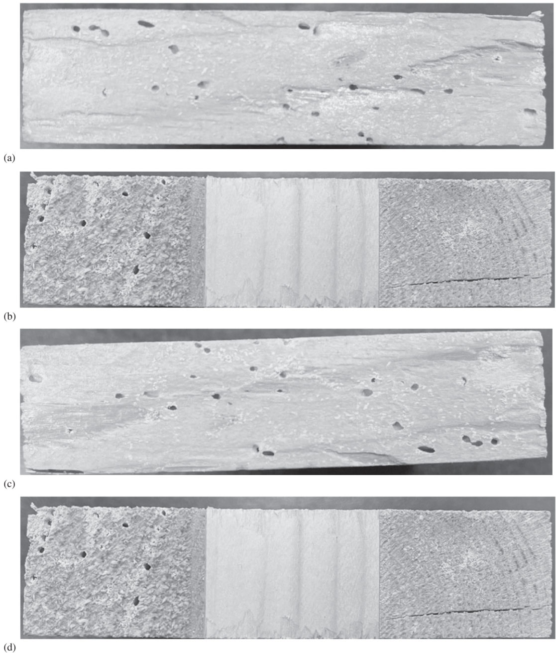
Figure 3. Example of termite damage on all sides of cross-laminated timber (CLT) samples from the test to evaluate termite number: with the top and bottom of the original panel (a and c), and the cut edges (b and d).
