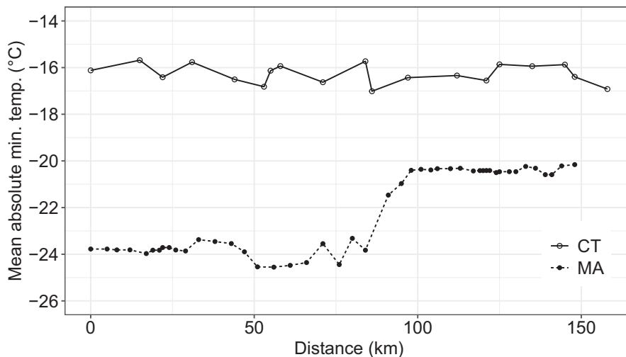
FIGURE 9 Mean absolute minimum temperatures as extracted from the PRISM data set for trap locations along the Massachusetts transect (dashed line) and the Connecticut transect (solid line) from 1 December through 31 March for 2007–2018. Distances are presented in relationship to T00 for the Massachusetts transect, and CT01 for the Connecticut transect
