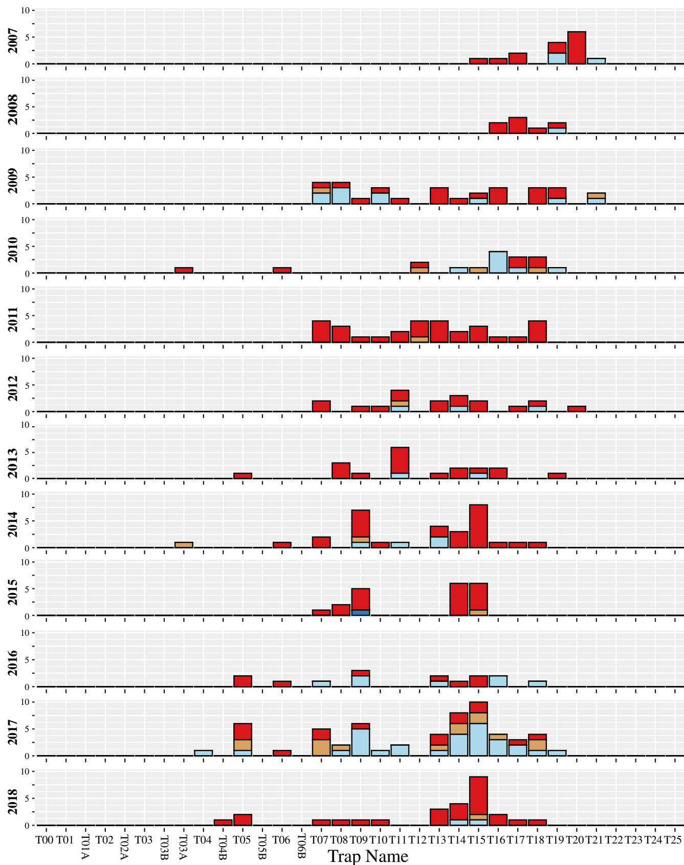
FIGURE 4 The number of genotyped individuals classified as F1 hybrids (red), F2 hybrids (orange), or winter moth backcrosses (blue) as calculated in NEWHYBRIDS [Colour figure can be viewed at wileyonlinelibrary.com ]
