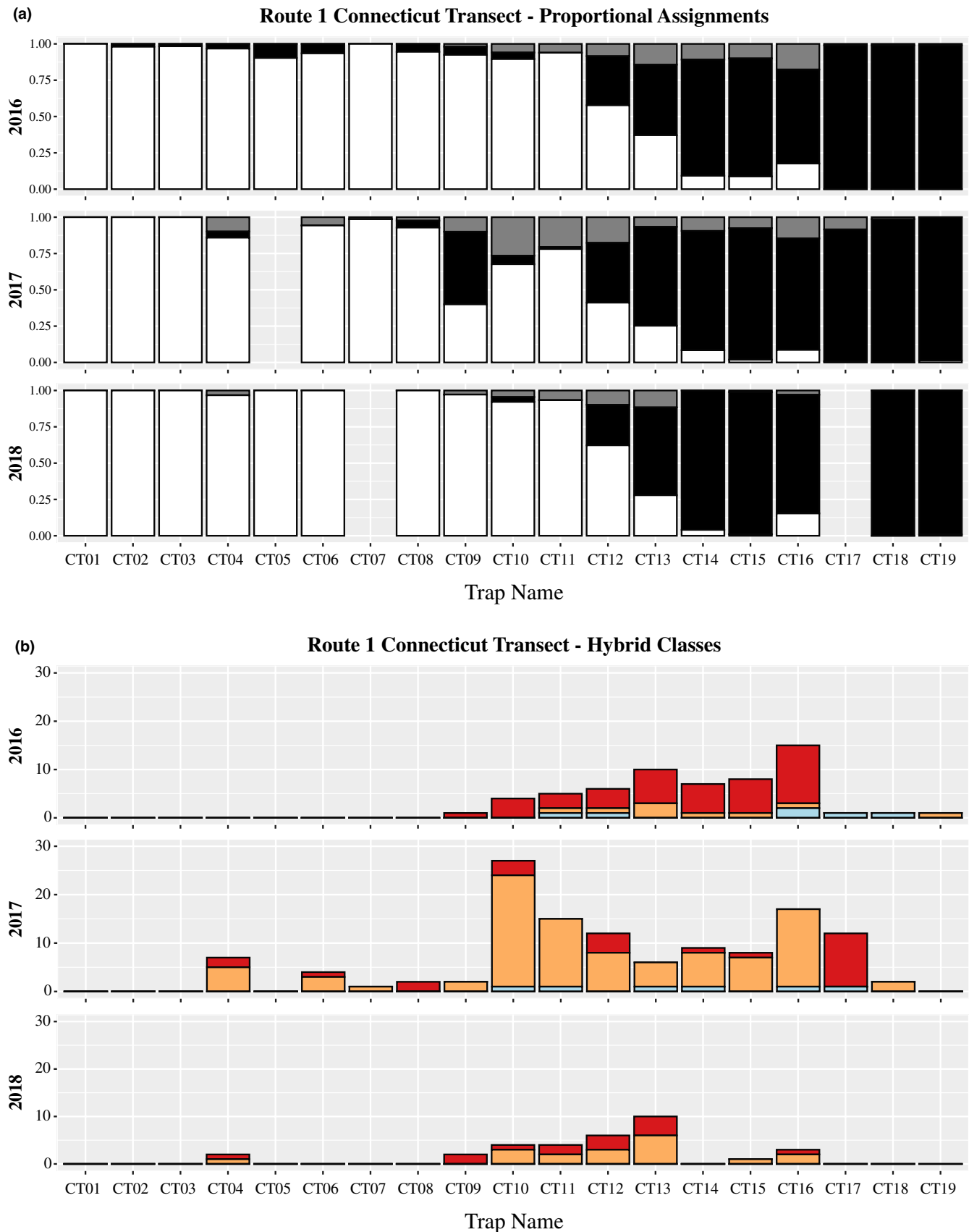
FIGURE 3 Proportional assignment of individuals collected along the Connecticut transect as either pure winter moth (black), pure Bruce spanworm (white), or to one of four hybrid categories (grey) in NEWHYBRIDS (a). The number of genotyped individuals classified as F1 hybrids (red), F2 hybrids (orange), or winter moth backcrosses (blue) are presented in (b) [Colour figure can be viewed at wileyonlinelibrary.com ]
