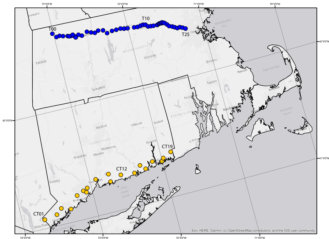
FIGURE 1 Locations of survey traps along the Massachusetts transect (blue) and the Connecticut transect (yellow). The western and eastern most points along each transect are labelled for reference, as are the traps most proximal to the centre of the hybrid zone in 2018 [Colour figure can be viewed at wileyonlinelibrary.com ]
