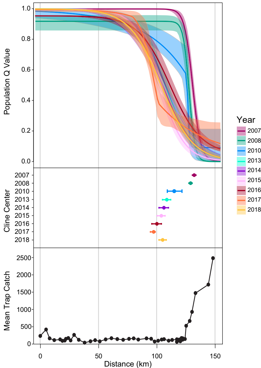
FIGURE 7 Cline analysis showing the fit of the best model based on the proportional assignment of populations to the Bruce spanworm genetic cluster (Q) for each sampled year along the Massachusetts transect (top) and the geographic centre \pm 2LL as estimated in the R package hzar (middle). The number of individuals collected at each trap averaged across the 2007–2018 sample years (bottom). Distances are presented in relationship to T00 [Colour figure can be viewed at wileyonlinelibrary.com ]
