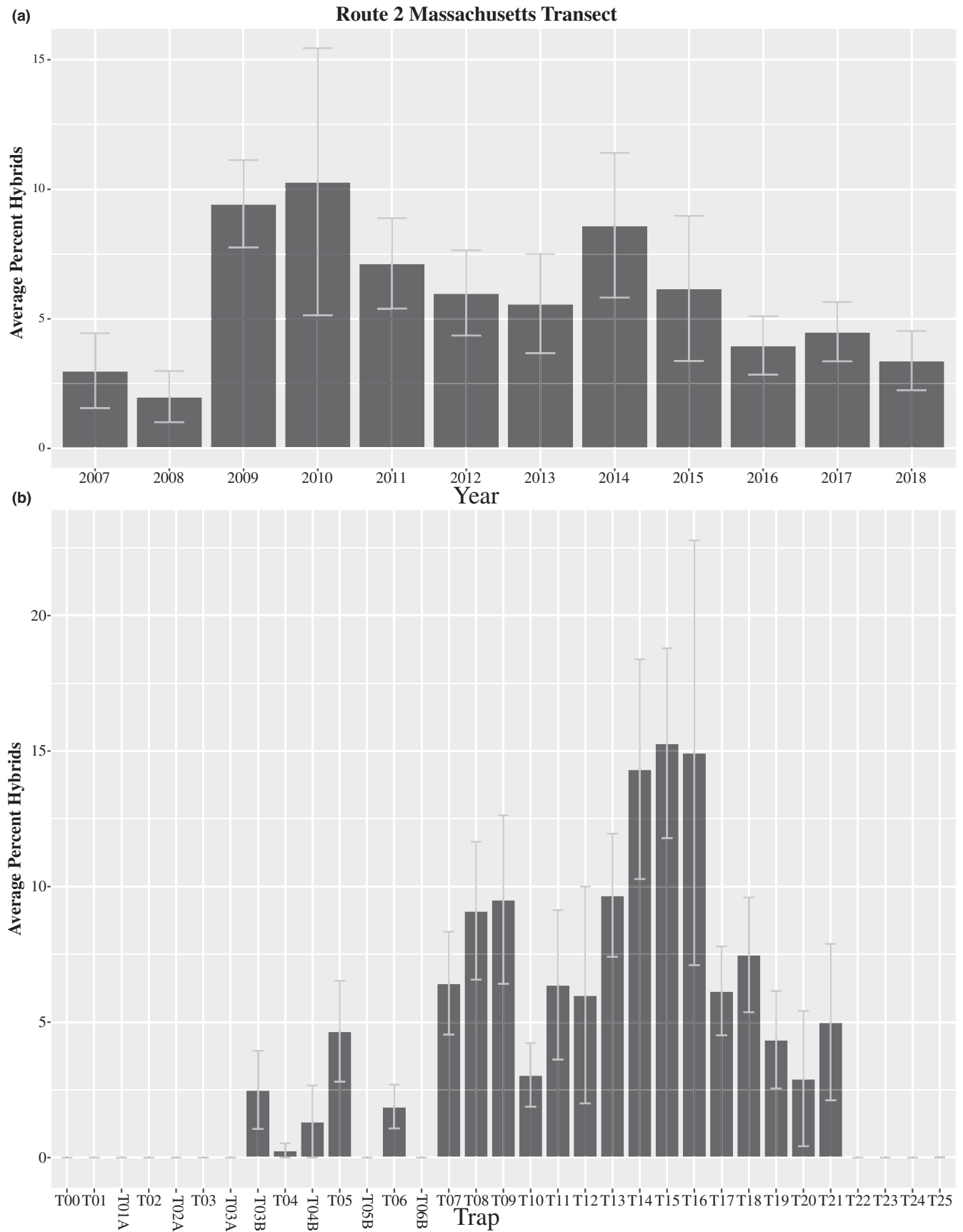
FIGURE 5 The average percentage ( \pm SE) of genotyped individuals classified as hybrids in 2007–2018 (a), and the average percentage ( \pm SE) of genotyped individuals classified as hybrids at each trap (b) for all years across the Massachusetts transect
