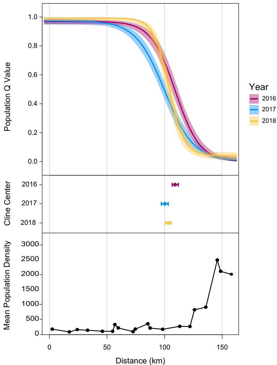
FIGURE 8 Cline analysis showing the fit of the best model based on the proportional assignment of populations to the Bruce spanworm genetic cluster (Q) for each sampled year along the Connecticut transect (top) and the geographic centre \pm 2LL as estimated in the R package hzar (middle). The number of individuals collected at each trap averaged across the 2016–2018 sample years (bottom). Distances are presented in relationship to CT01 [Colour figure can be viewed at wileyonlinelibrary.com ]
