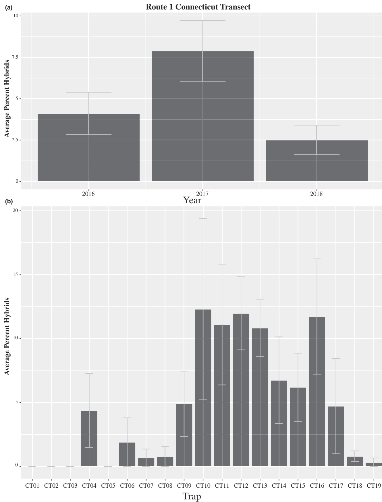
FIGURE 6 The average percentage ( \pm SE) of genotyped individuals classified as hybrids in 2016–2018 (a), and the average percentage ( \pm SE) of genotyped individuals classified as hybrids at each trap (b) for all years across the Connecticut transect
