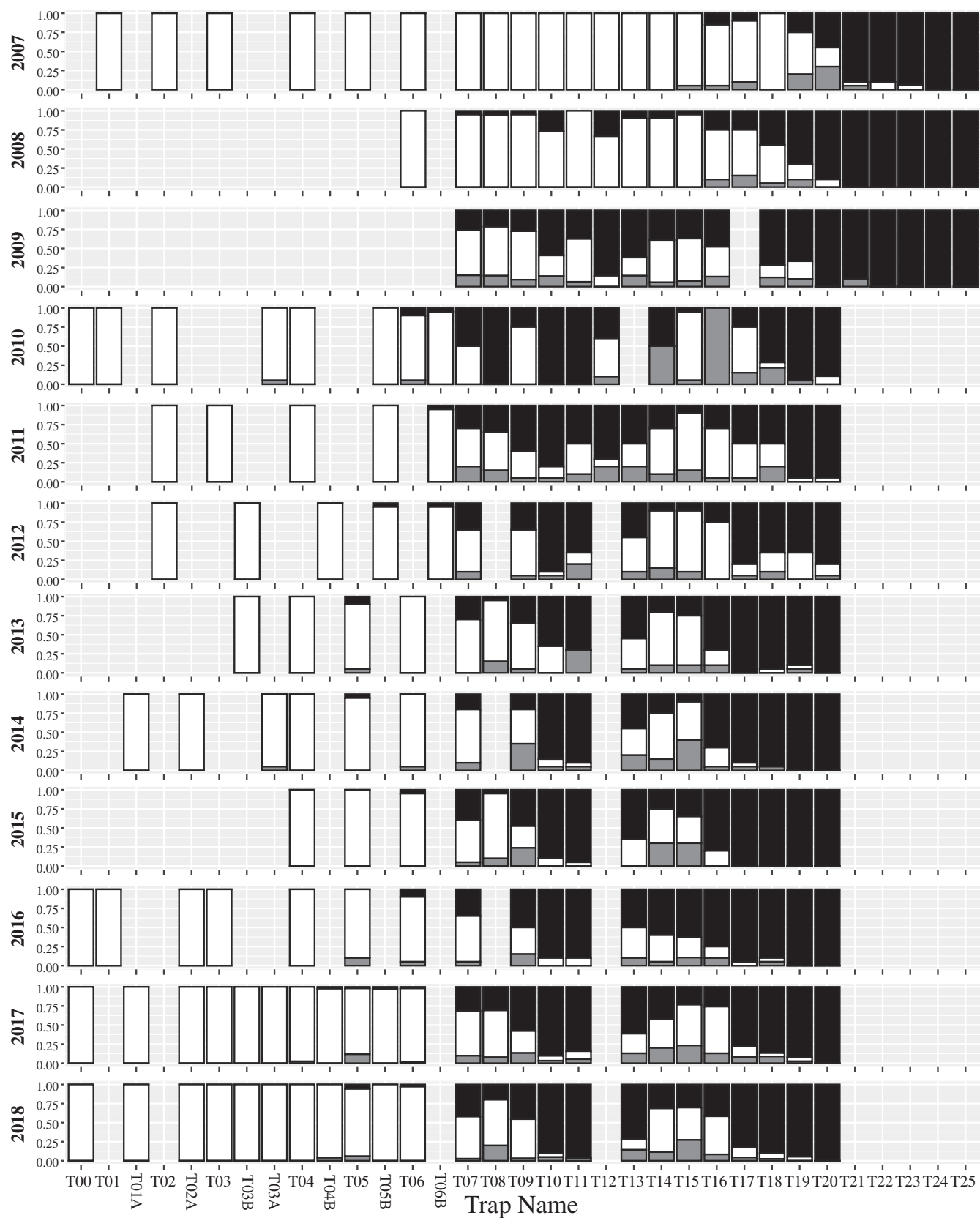
FIGURE 2 Proportional assignment of individuals collected along the Massachusetts transect as either pure winter moth (black), pure Bruce spanworm (white), or to one of four hybrid categories (grey) in NEWHYBRIDS
