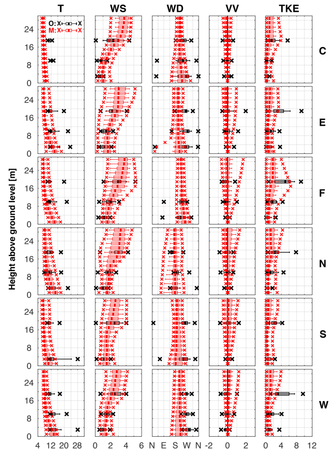
Figure 5. Box and whisker plot vertical profiles of 1 min mean temperature ( T ; ^{\circ}\text{C} ), wind speed ( WS ; \text{m s}^{-1} ), wind direction ( WD ; ^{\circ} ), vertical velocity ( VV ; \text{m s}^{-1} ), and turbulent kinetic energy ( TKE ; \text{m}^2 \text{s}^{-2} ) for the control simulation (HFP 2.4L ) at all towers (labeled along the right axis). Box and whisker plots are constructed from 40 1 min mean values \pm 20 min from the time of peak 1 min mean observed heat flux, except for TWR C , wherein 15:20 EDT is chosen arbitrarily; TWR E is centered at 15:42 EDT, TWR F is centered at 15:28 EDT, TWR N is centered at 16:20 EDT, TWR S is centered at 15:08 EDT, and TWR W is centered at 15:38 EDT. For each box and whisker plot, the thick line denotes the median, the boxes extend outward to the 25th and 75th percentiles, the whiskers extend outward to the 10th and 90th percentiles, and the “x” symbols indicate the minimum and maximum values. Tower observations ( O ) and model-simulated values ( M ) are indicated by black and red colors, respectively (see the legend in the top-left panel). The vertical black line in the VV column corresponds to zero vertical velocity. The x axis in the WD column is labeled as follows: N ( 0/360^{\circ} ), E ( 90^{\circ} ), S ( 180^{\circ} ), W ( 270^{\circ} ). Manual quality control of tower observations results in the exclusion of three data points: lower tower level T at TWR C and TWR F and upper tower level WD at TWR F .
