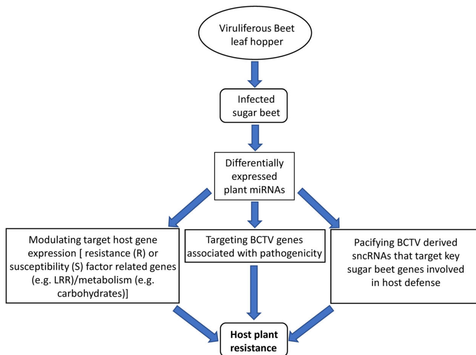
FIGURE 8 | Proposed model of miRNA mediated sugar beet resistance against BCTV in the resistant genotypes.
