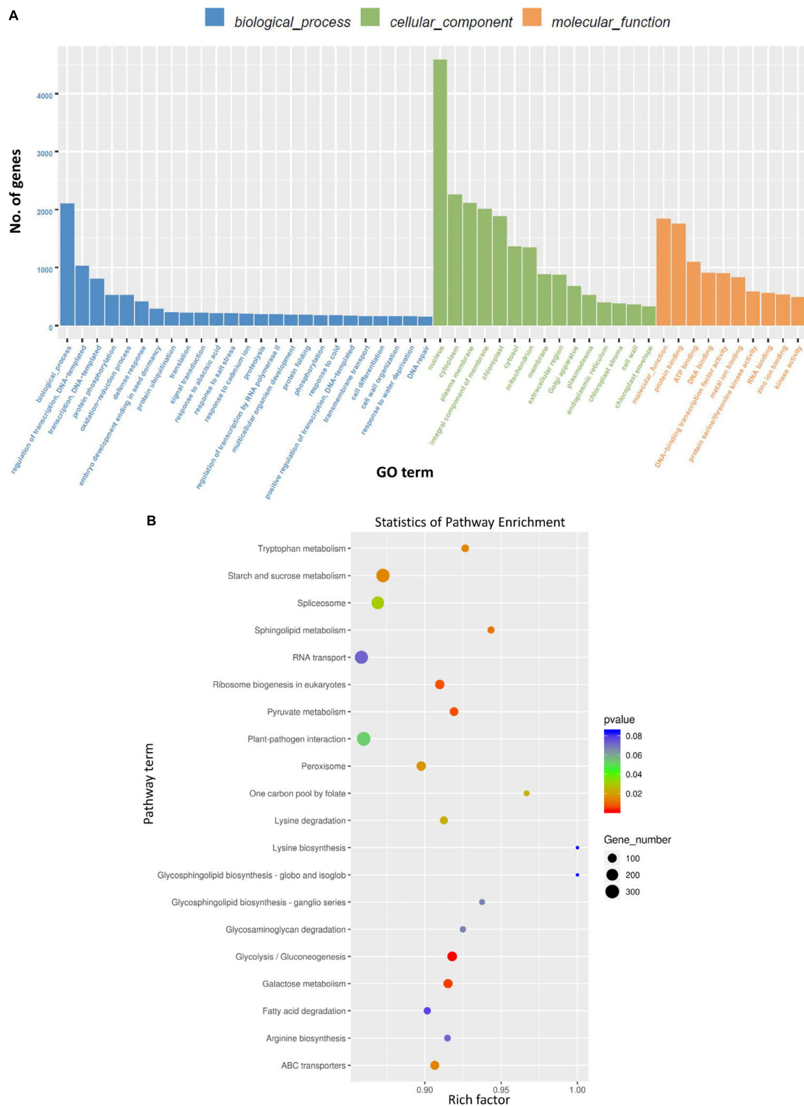
FIGURE 4 | Gene ontology (GO) term and Kyoto Encyclopedia of Genes and Genomes (KEGG) enrichment of the sugar beet gene targets of differentially expressed (DE) sugar beet miRNAs in leaves. (A) GO annotation of sugar beet gene targets of DEMiRNAs in leaves, and (B) KEGG enrichment of sugar beet gene targets of DEMiRNAs.
