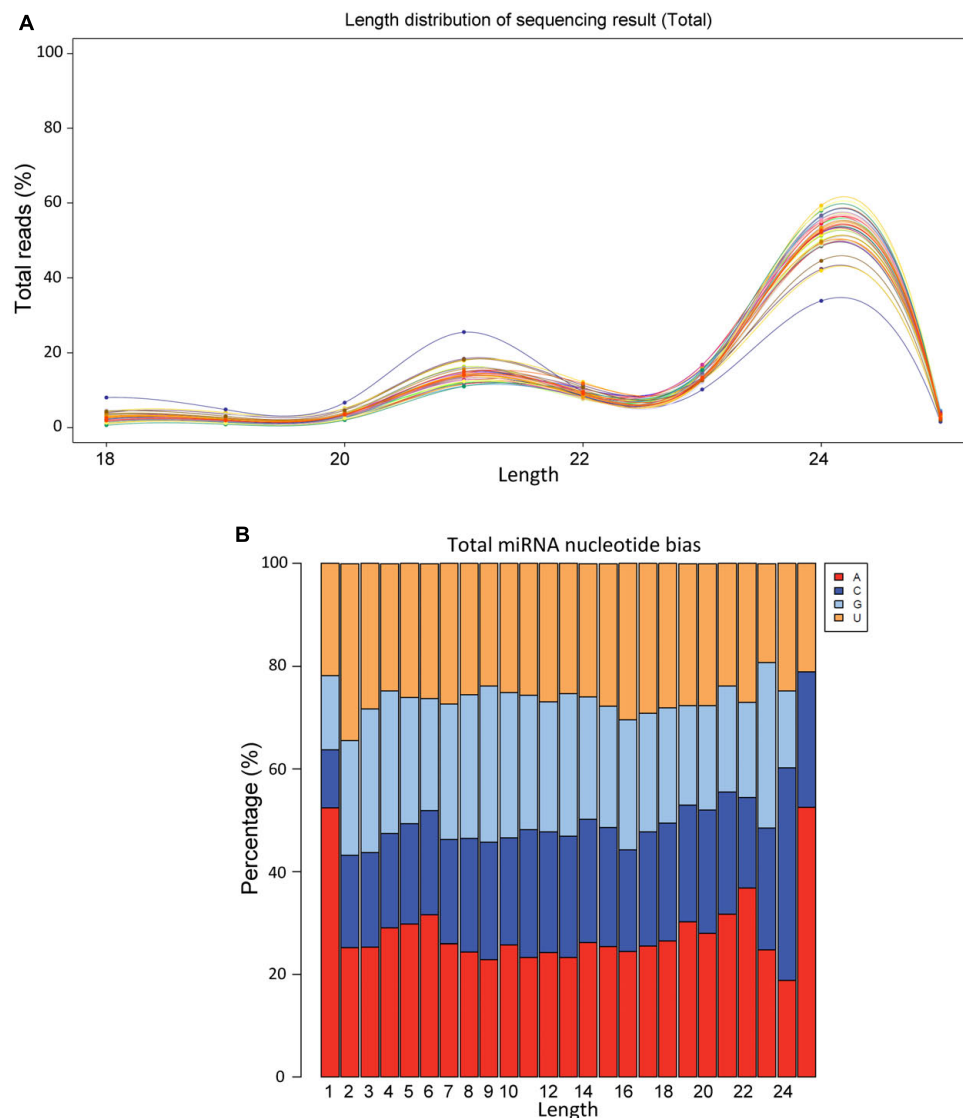
FIGURE 1 | Size distribution and nucleotide bias of miRNAs derived from sugar beet leaves. (A) Size distribution and (B) nucleotide bias.
