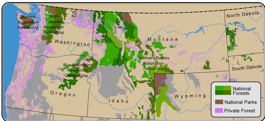
Fig. 1 Locations of the national forests and national parks involved in four climate change adaptation partnerships in the western United States. Private lands in the region are shown in pink , and other national forests (not involved in the assessments described here) are shown in gray . Map by R. Norheim
