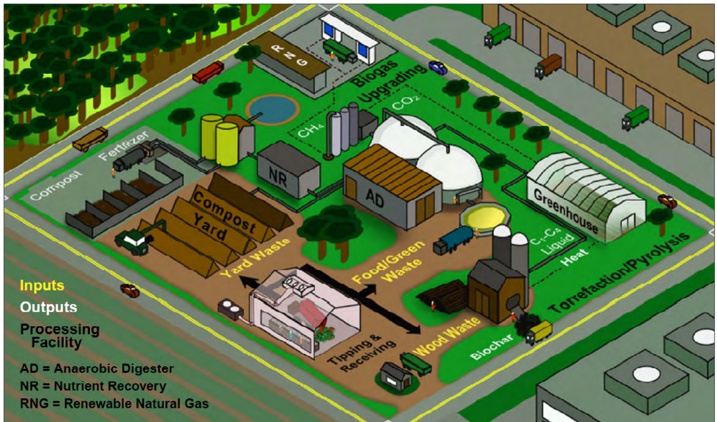
Figure 7.7. The biorefinery concept for processing organic waste (Source: Hills et al. 2019).
