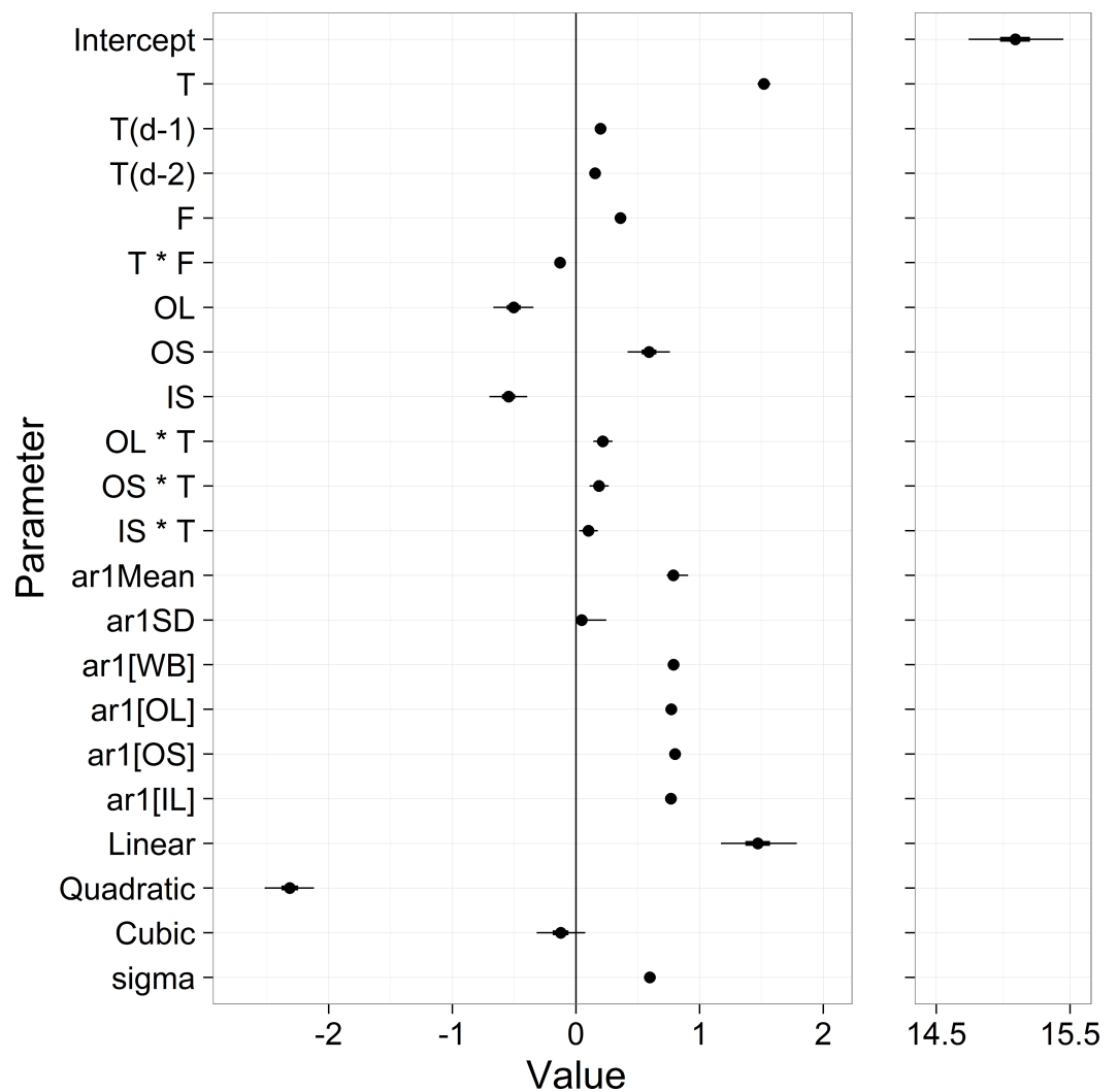
Figure 5 Parameter estimates from the stream temperature model. ‘T’ stands for temperature, ‘F’ stands for flow, and OL, OS, IL are streams. The first 12 rows represent the \beta_x in Eq. (5). ‘ar1[x]’ are the \delta_x from Eq. (3), and the ‘Linear’, ‘Quadratic’ and ‘Cubic’ parameters are the \mu Y_x from Eq. (7). ‘sigma’ is the residual standard deviation from Eq. (1).
