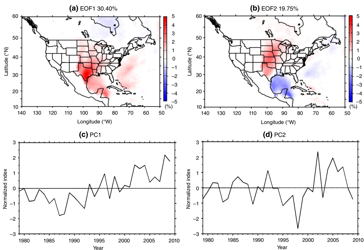
Figure 3. Spatial patterns (panels a and b) and time series of the corresponding principal components (panels c and d) of the two leading EOF modes of SLLJ frequency during the warm season for 1979–2009.
