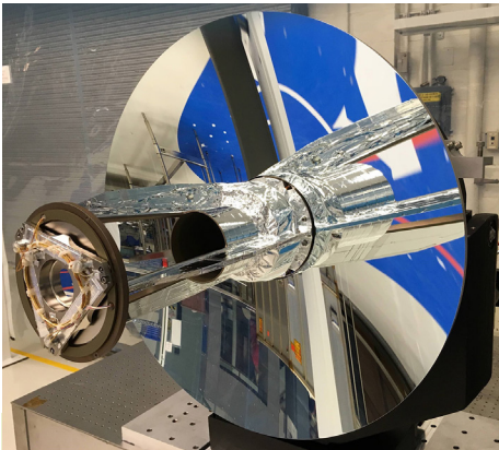
The Global Ecosystem Dynamics Investigation (GEDI) LiDAR is the highest resolution LiDAR system ever deployed from space. Pictured is the 80-cm telescope that will collect the returned pulses. The system was launched on December 5, 2018 and began formally collecting sample data in spring 2019. The University of Maryland is leading the project in collaboration with the NASA Goddard Space Flight Center.
