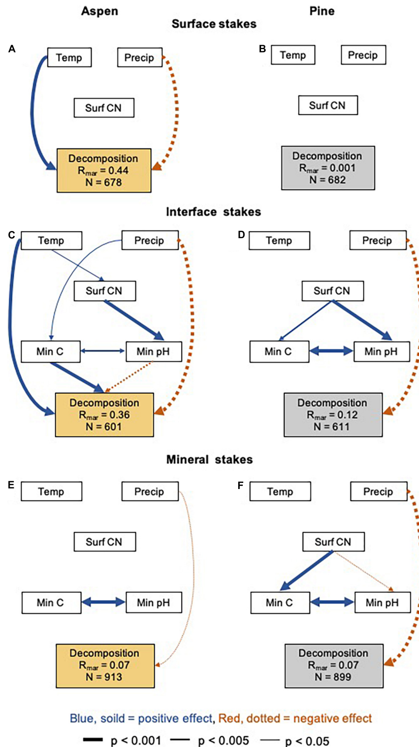
FIGURE 3 | Influence of local environmental conditions on the wood decomposition (mass loss in %) in forested ecosystems. Structural equation model (SEM) diagrams illustrate climatic and soil properties found to affect decomposition of (A) surface aspen stakes, (B) surface pine stakes, (C) interface aspen stakes, (D) interface pine stakes, (E) mineral aspen stakes, (F) mineral pine stakes. Blue, solid lines represent positive relationships, red, dashed lines negative relationships. Line width corresponds to differences in significance levels (thick = p < 0.001 , medium = p < 0.005 , thin = p < 0.05 ). Non-significant connections were removed. Temp, average air temperature per site for the individual incubation time per wood stake; Precip, average precipitation per site for the individual incubation time per wood stake; Surf CN, surface organic horizon C:N ratio; Min C, mineral soil C concentration; Min pH, mineral soil pH. Decomposition values were log-transformed. Total number of sites included for surface aspen and pine = 19, interface aspen and pine = 10, mineral soil aspen and pine = 23. For alternative models see
