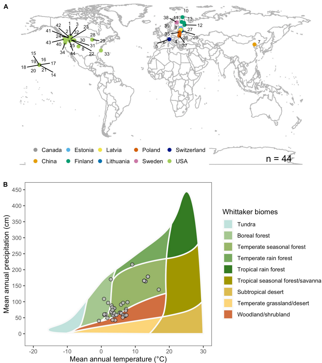
FIGURE 1 | Geographic and climatic distribution of experimental sites. (A) Locations of the 44 sites at which our decomposition experiments were conducted. (B) The sites cover all major forest biomes with the exception of tropical rainforests and tropical seasonal forests/savannas. Mean annual temperature (MAT) and mean annual precipitation (MAP) values represent 30-year mean values between 1970 and 2020. Data was obtained from the Worldclim data base ( www.worldclim.com ). Additional site details can be found in Supplementary Tables 1, 2 .
