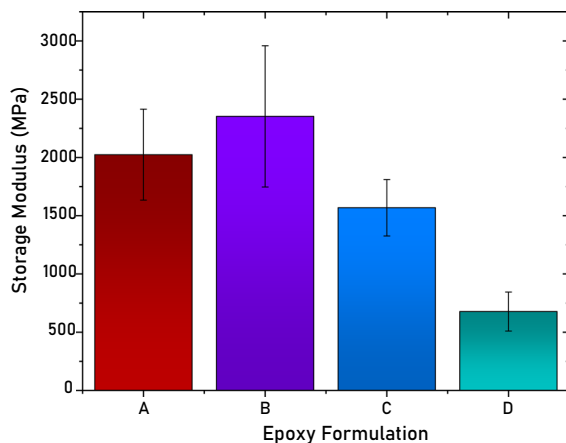
Fig. 5 Storage modulus of different epoxy formulations as taken from the DMA
