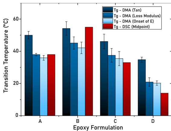
Fig. 4 Glass transition temperature of different epoxy formulations as taken from DMA and DSC
