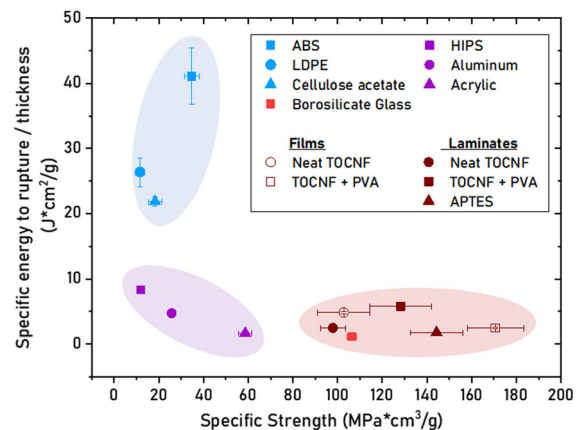
Fig. 8 Plot shows specific energy to rupture divided by thickness ( t ) against the specific strength of various materials, including ABS, LDPE, Cellulose acetate, Acrylic, PS, Aluminum, Borosilicate Glass, Neat TOCNF and TOCNF + PVA films and 3 different 10 layers TOCNF or TOCNF + PVA laminates. Blue bubble are ductile polymers (low specific strength but high specific energy to rupture), purple bubble somewhat brittle materials (low specific strength and energy to rupture), red bubble indicates high specific strength but low specific energy to rupture
