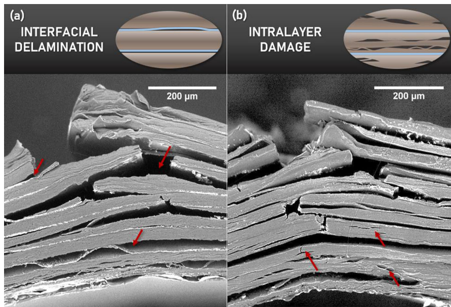
Fig. 3 Top schematics describe two different fracture behaviors (interfacial delamination vs intralayer damage) related to the SEM images of 10-layer TOCNF film laminates after loading/rupture. a Neat TOCNF—Epoxy A laminate, red arrows
