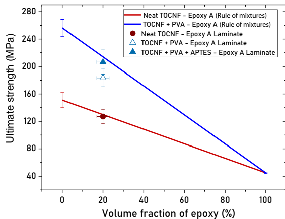
Fig. 7 Tensile testing of different laminates. Blue and red lines represent the iso strain rule of mixtures of TOCNF + PVA—Epoxy A and Neat TOCNF—Epoxy A laminates
