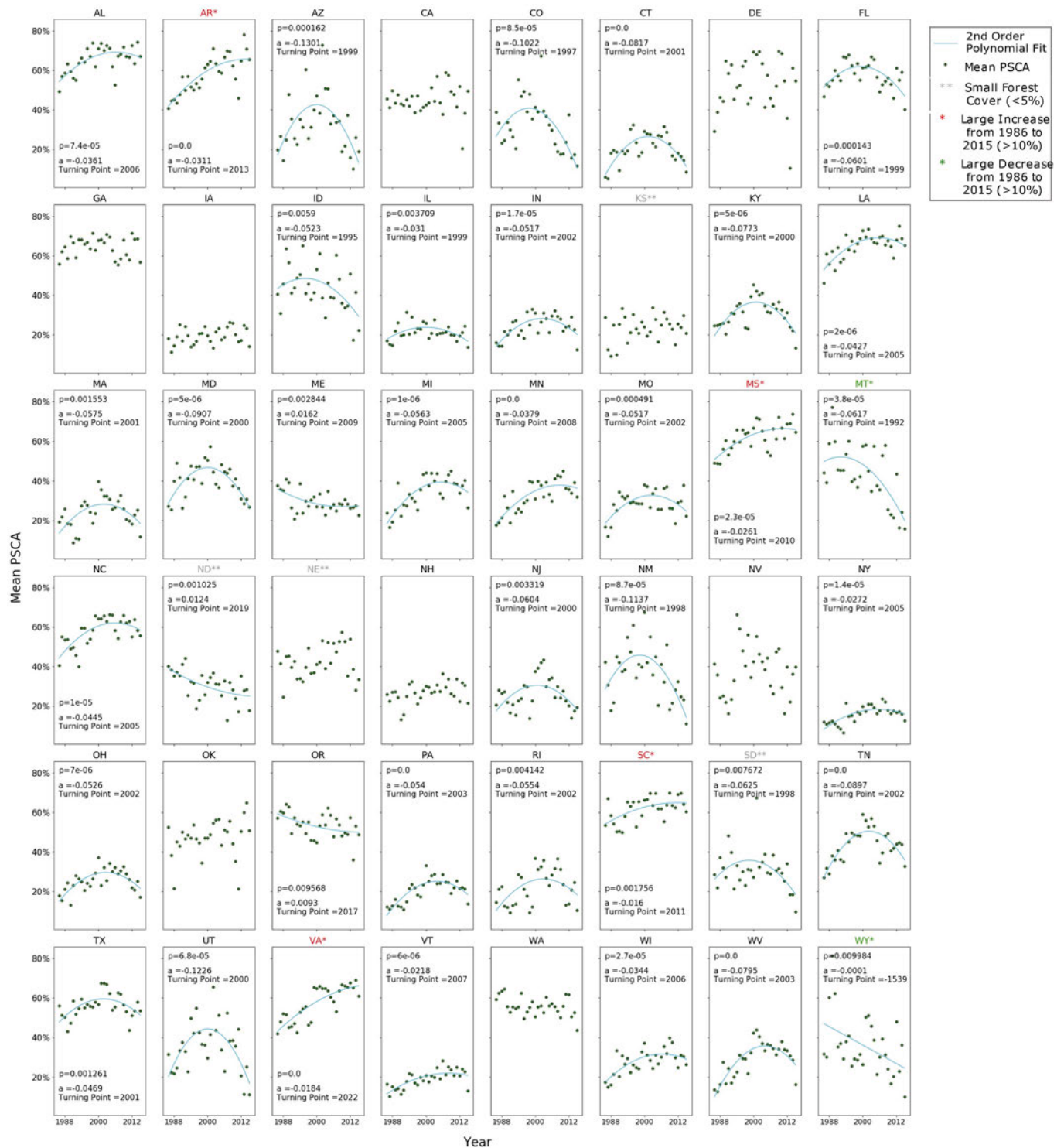
Fig. A3. Temporal profiles of average PSCA in CONUS states. Second order polynomial trend lines (blue curve) are plotted where significant trend is fitted. (For interpretation of the references to colour in this figure legend, the reader is referred to the web version of this article.)
