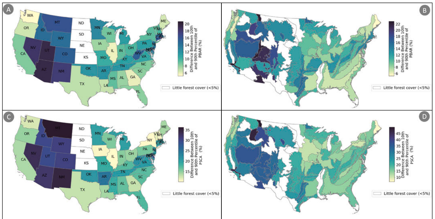
Fig. 9. Temporal range of state level mean annual PBAR calculated as the difference between the annual mean PBAR values (A: of each state; B: of each ecoregion) and PSCA values (C: of each state; D: of each ecoregion) at the 90th and 10th percentiles.
