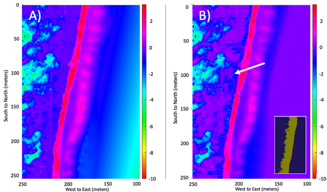
Fig. 6. Case study T_0 to T_1 , (A) actual topographic change pre- to post-Sandy (DEM T_0 - T_1 ) versus (B) simulation post-Sandy differences ( T_{1Sim} - T_{1Actual} ) (B). Regarding performance, the model over-estimated foredune erosion (too much dune transgression). However, the overall broader erosion patterns regarding swale deepening and beach erosion are congruent with reality, just more conservative in the simulation. Negative values reflect T_0 (A) or T_{1Sim} (B) having lower elevation than in T_1 (A) and T_{1Actual} (B), respectively. Positive values reflect a cell T_0 (A) and T_{1Sim} (B) that was taller pre-storm and eroded in the storm. For orienting, the B inset graph depicts the beach in yellow, and dune and ocean east and west of the beach. *Colorbars to the same scale. The arrow in B denotes the area that was over-transgressed by the storm sub-model T_0 to T_1 which largely lacked vegetation the rest of the simulation. (For interpretation of the references to colour in this figure legend, the reader is referred to the web version of this article.)
