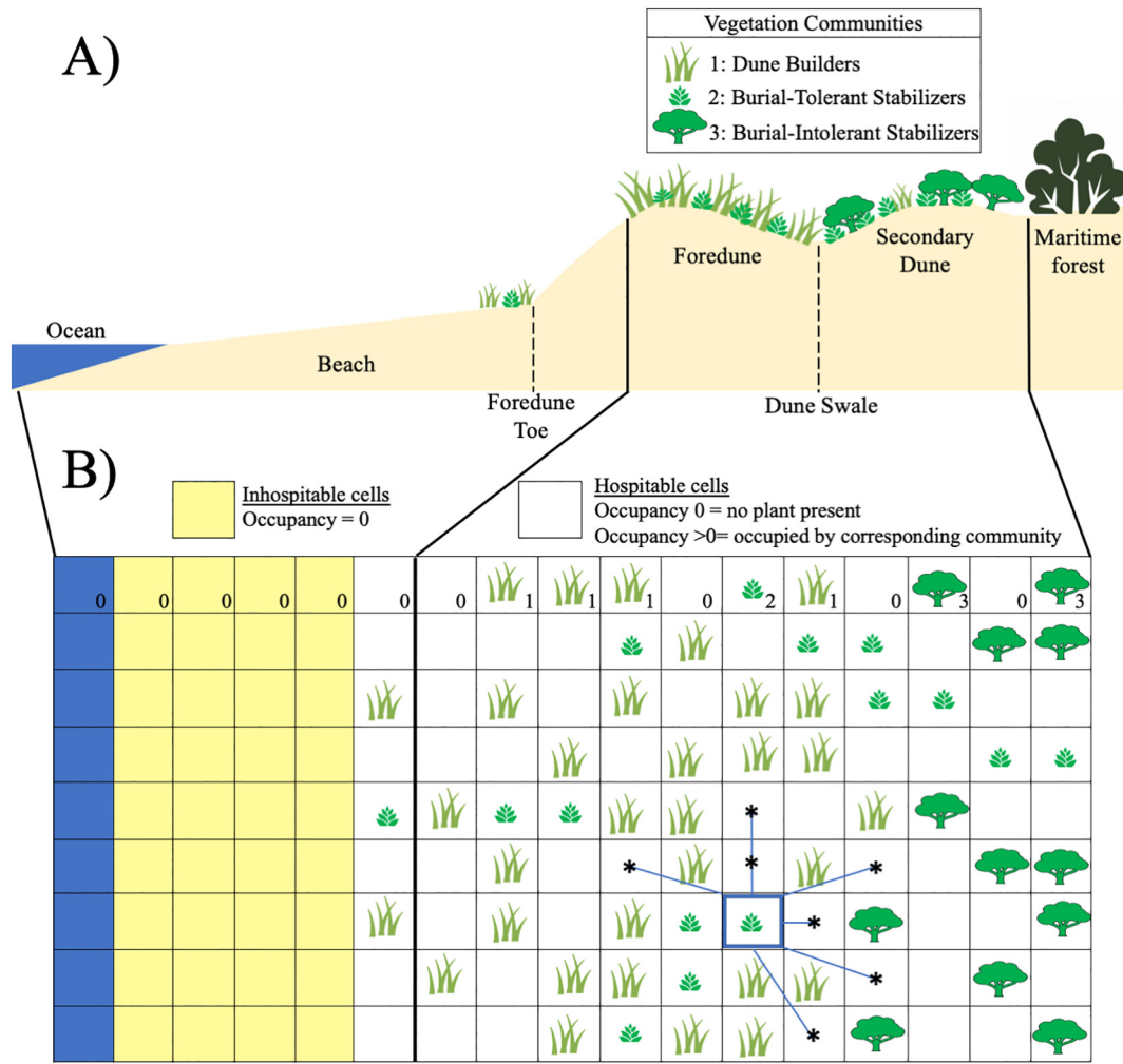
Fig. 2. The coastal dune habitat. (A) A cross section and overhead (B) conceptualization with the three vegetation functional types and their expected relative distributions within the habitat. (B) DOONIES is grid-based, and vegetated cells represent super-individuals that can disperse asexually into unoccupied cells within their lateral expansion range.
