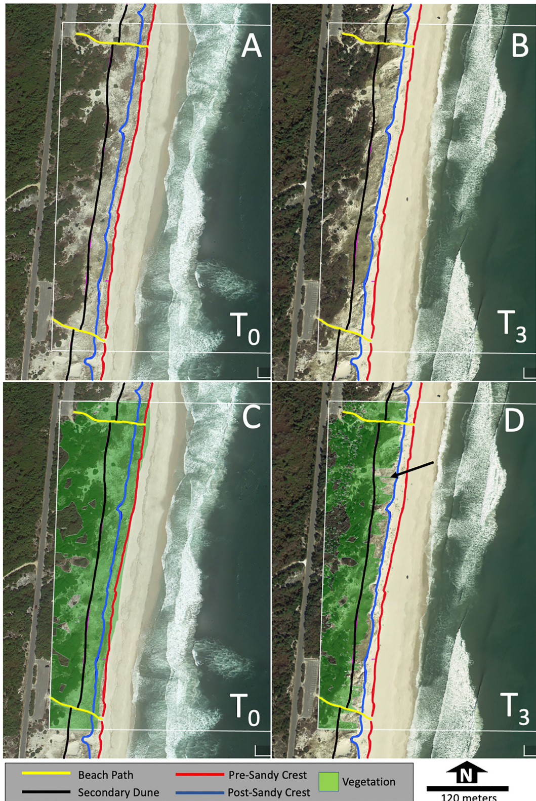
Fig. 9. Vegetation in reality (A & B) versus the simulation (C & D) during the full case study duration from T_0 pre-Hurricane Sandy to T_3 5-yrs post-Sandy September 2017. Initial vegetation placement T_0 closely mirrored reality comparing A and C, largely spanning the full dune habitat from the pre-Sandy dune crest landward. At the simulation end (B & D), vegetation remains largely absent between the pre- and post-Sandy crest, except in isolated small patches where dispersal occurred. Denuded areas landward of the pre-Sandy crest where vegetation would be expected in reality stem from over-transgression T_0 to T_1 from the storm sub-model and subsequent slow recovery in re-establishment of vegetation in storm denuded areas. The aeriels are projected and pulled from Google Earth View Pro for September 2010 (time soonest T_0 when flight was flown when plants were green and expanded) and October 2017 (one month after actual T_3 ) reflecting T_0 and T_3 , respectively and line layers were mapped in the field (Charbonneau et al., 2017). The arrow in D denotes the area that was over-transgressed by the storm sub-model T_0 to T_1 which largely lacked vegetation the rest of the simulation.
