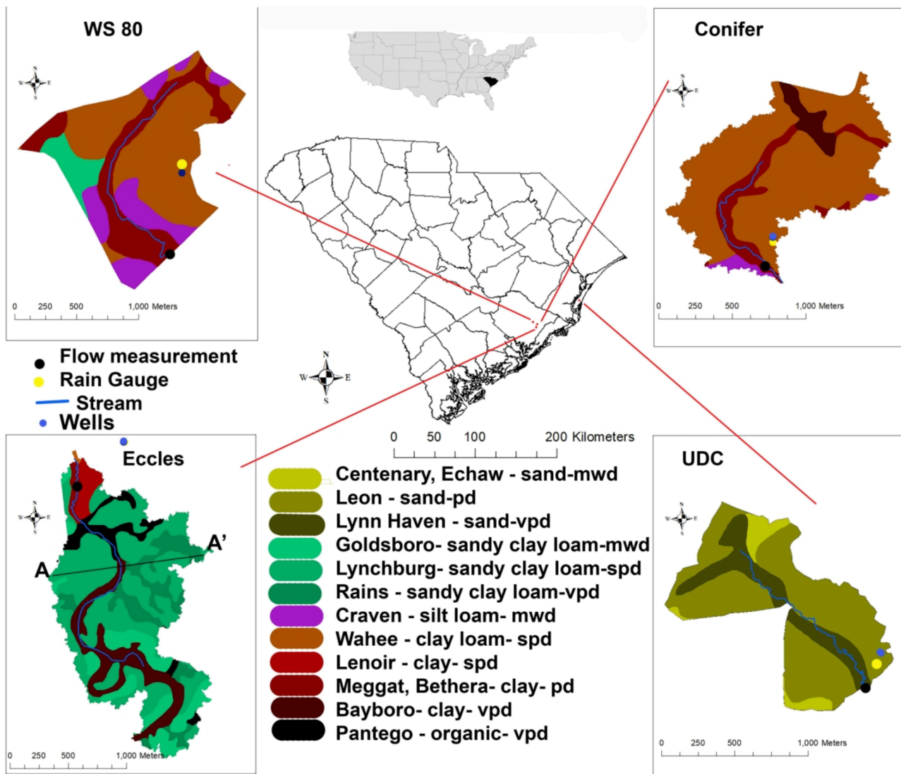
Fig. 1. Location and soil distribution maps for WS80, Conifer, Eccles Church, and UDC watersheds with their wells, rain gauges, and flow gauging stations. Listed for each soil is the soil series name, subsurface soil texture, and soil drainage class ( mwd -moderately well drained, spd - somewhat poorly drained, pd - poorly drained, vpd -very poorly drained). Note line A-A' is used in Fig. 9 below.
