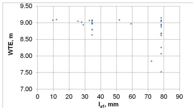
Fig. B2. Relationships between WTE and I_{a1} in WS80 watershed
