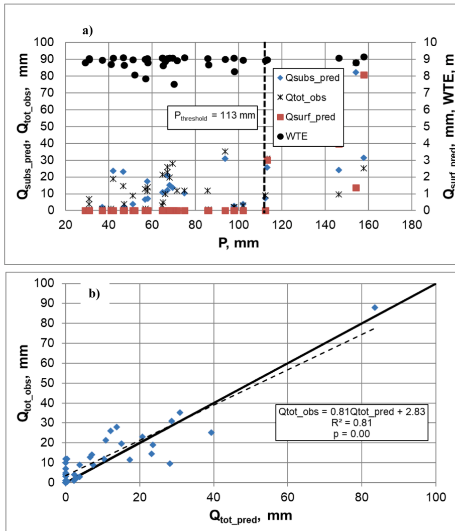
Fig. 4. Relationships for the WS80 watershed between a) measured event total rainfall ( P ) and observed direct runoff ( Q_{tot\_obs} ), predicted saturated subsurface runoff ( Q_{subs\_pred} ), predicted overland surface runoff ( Q_{surf\_pred} ) and water table elevation (WTE) and b) Q_{tot\_obs} and predicted runoff ( Q_{tot\_pred} ) for rainfall-runoff events, with a solid black line for 1:1 relationship. The dashed line in Fig. 4b represents the regression line with R^2 (coefficient of determination) and a p value.
