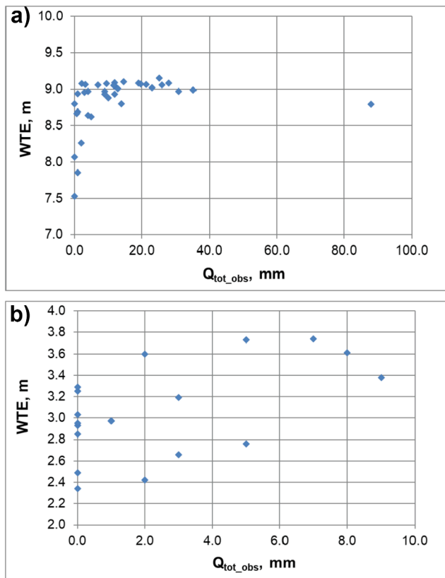
Fig. 8. Relationship between WTE and observed total runoff for a) WS80 and b) UDC watersheds.
