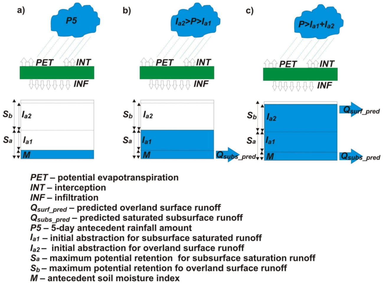
Fig. 2. A conceptual diagram of components of direct runoff formation in the MSME model.
