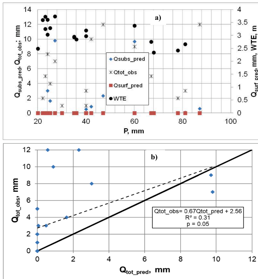
Fig. 7. Relationships for the UDC watershed between: a) measured total event rainfall ( P ) and predicted total surface runoff ( Q_{tot\_pred} ) and its components and b) relationship between Q_{tot\_obs} and Q_{tot\_pred} for rainfall-runoff events, with a solid black line for 1:1 relationship. The dashed line in Fig. 7b represents the regression line with R^2 (coefficient of determination) and a p value.
