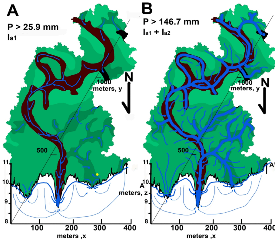
Fig. 9. Conceptual diagram of runoff generation on a pseudo-3D representation of the Eccles Church watershed. MSME model estimates of initial abstraction (average values of I_{a1} and I_{a2} in Table 5) are related to: A) situation where only subsurface runoff occurs near the channel and B) where streamside runoff extends, by an expanding channel system, across most of the watershed to become watershed-wide overland surface runoff. Arrow sizes reflect the volume of runoff. This figure is derived from Fig. 1c as a cross-section relating to transect line A-A' and a plan view upstream to the south.
