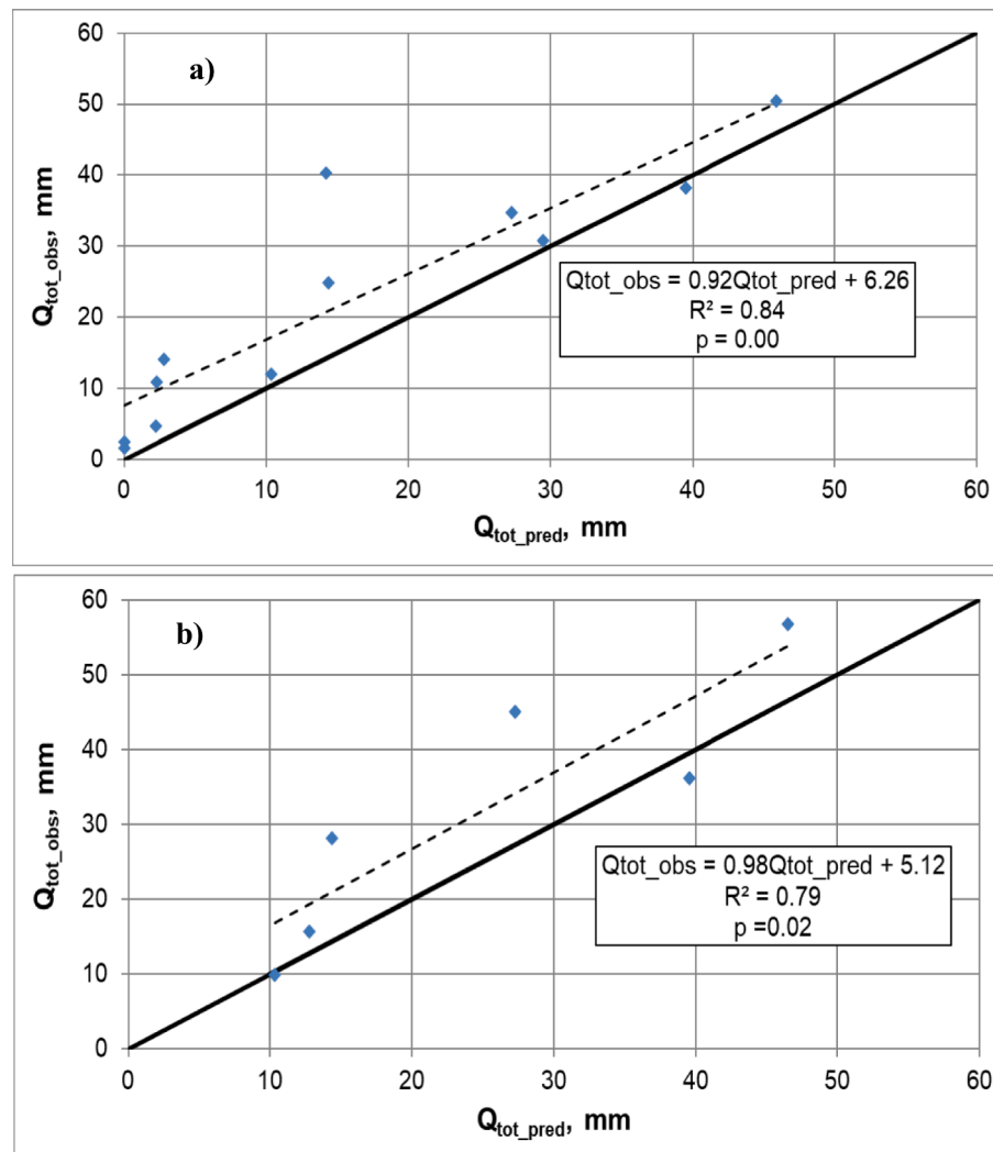
Fig. 6. Relationship between Q_{tot\_obs} and Q_{tot\_pred} for rainfall-runoff events on a) Eccles Church and b) Conifer watersheds. The solid black lines represent a 1:1 relationship and the dashed lines represent regression lines with R^2 (coefficient of determination) and p value.
