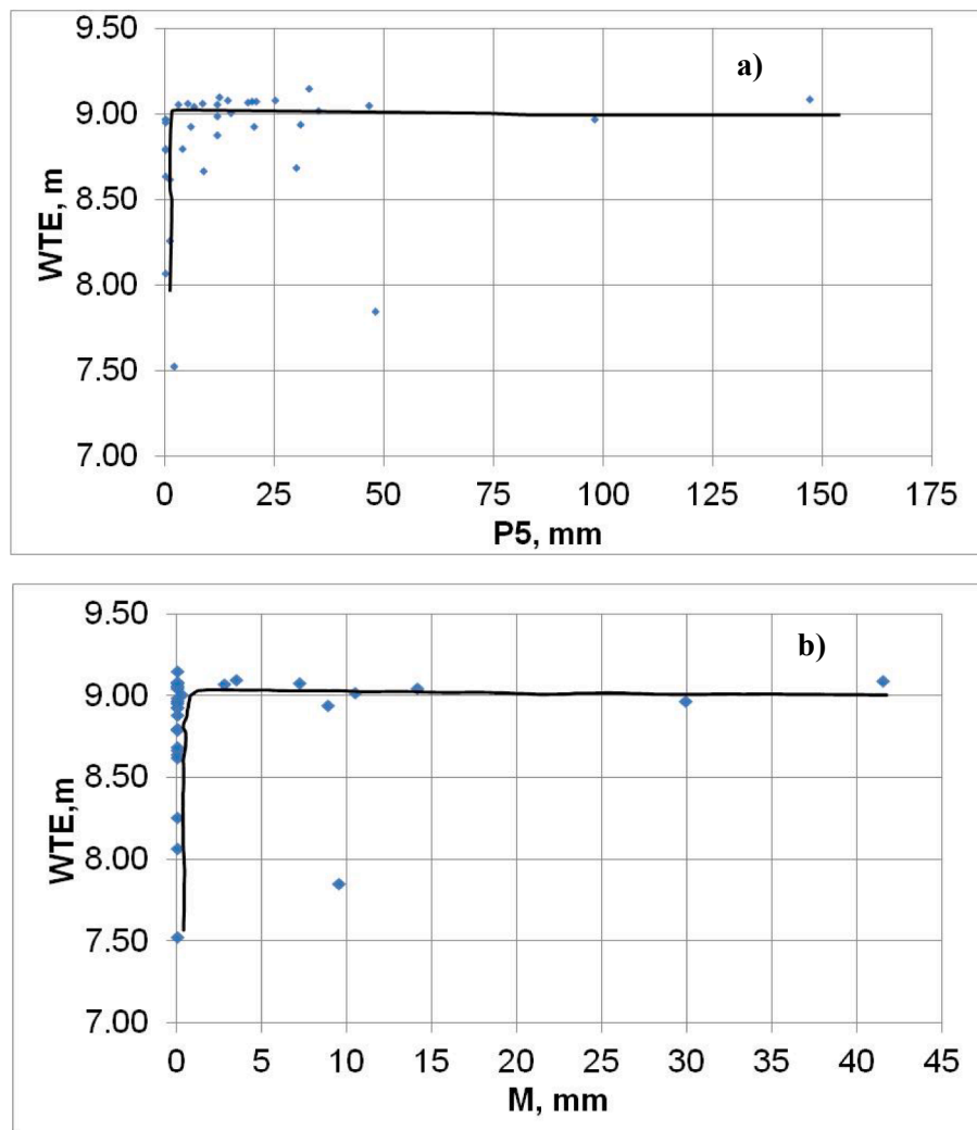
Fig. 3. Relationships between a) water table elevation (WTE) and P_5 and b) WTE and antecedent soil moisture ( M ) on WS80 watershed; the solid black line represents the average fitted relationship.
