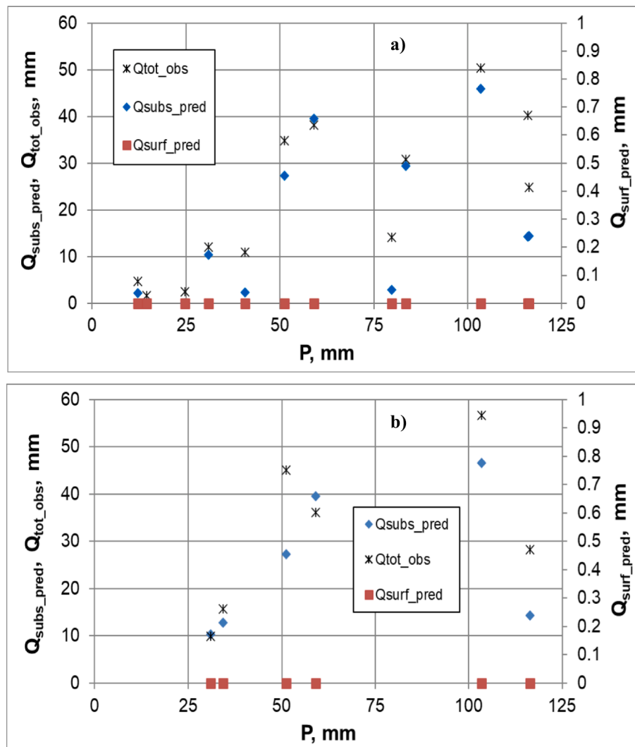
Fig. 5. Relationships between measured event total rainfall ( P ) and observed direct runoff ( Q_{tot\_obs} ), predicted saturated subsurface runoff ( Q_{subs\_pred} ), and predicted overland surface runoff ( Q_{surf\_pred} ) for a) Eccles Church and b) Conifer watersheds.
