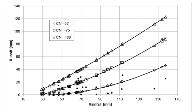
Fig. B1. The observed rainfall-runoff events and direct outflow calculated according to SCS-CN method for different CN values, corresponding to three antecedent moisture conditions for WS80 watershed.
