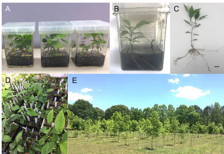
Fig. 7 White and green ash somatic seedlings derived from lingering ash sources. (a) Lingering white ash somatic seedlings of genotype LA112-10 following cold treatment and germination on medium with activated charcoal and GA_3 . (b) Somatic seedling derived via in vitro conversion after 10 weeks. (c) Somatic seedling derived via ex vitro conversion after 10 weeks. Bar = 1 cm. (d) Somatic seedlings from embryogenic cultures derived from control-pollinated seeds from crosses between two lingering green ash parents (DC4×DC2) in the greenhouse. (e) Field test of lingering ash somatic seedlings and controls in Athens, GA in the second growing season (May 2021)
