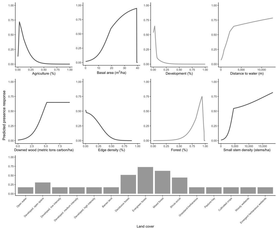
FIGURE 3 Response curves for predictor variables used in maximum entropy (MaxEnt) modeling of plains spotted skunk distribution in Arkansas and Missouri, USA, 1999–2019. Response curves are based on univariate models to prevent collinearity among variables from affecting the relationships shown. Response curves in gray represent those variables that remained in the simple multivariate MaxEnt model. Line graphs represent continuous variables and bar graphs represent categorical variables
