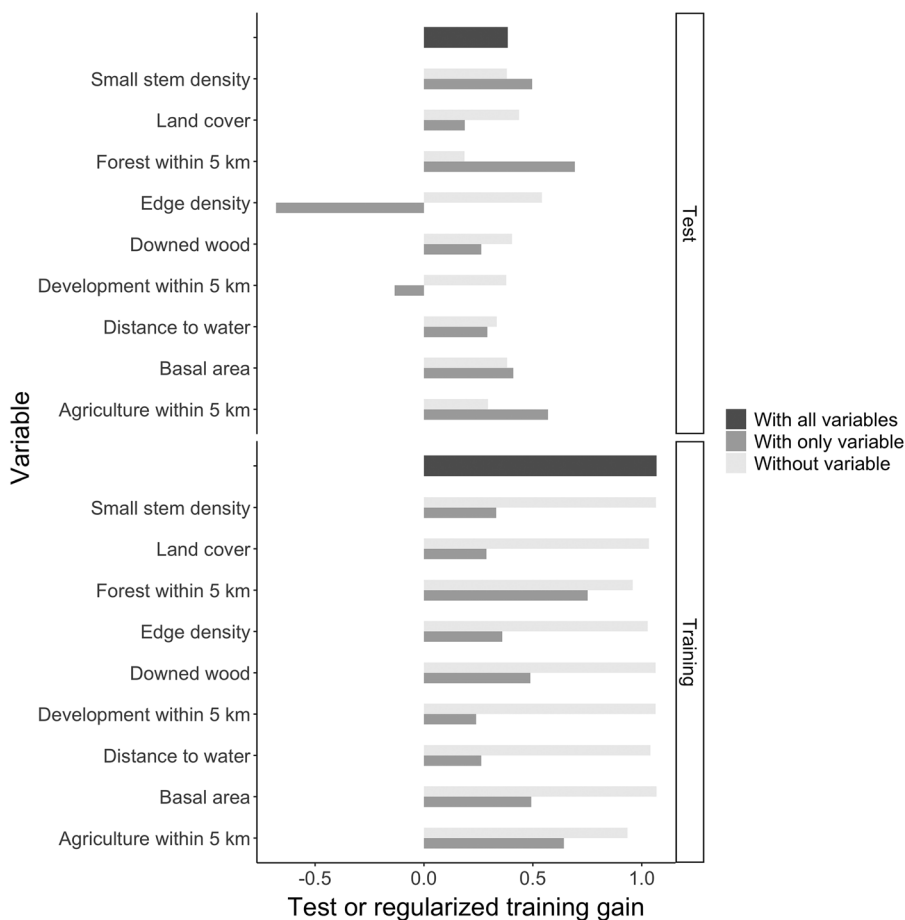
FIGURE 2 Test (top) and regularized training (bottom) gain variables in the full multivariate maximum entropy (MaxEnt) model of plains spotted skunk distribution in Arkansas and Missouri, USA, 1999–2019. High gain in a univariate model (with only variable) indicates the variable was more important to the model, while high gain in a model without the variable (without variable) indicates lower importance. The large dark gray bar (with all variables) represents test or training gain for the model including all variables for the test and training datasets, respectively
