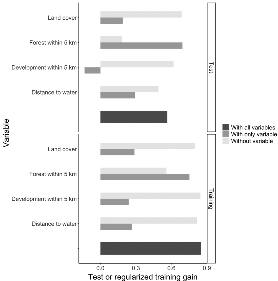
FIGURE 1 Test (top) and regularized training (bottom) gain for variables that remained in the simple multivariate maximum entropy (MaxEnt) model of plains spotted skunk distribution in Arkansas and Missouri, USA, 1999–2019. High gain in a univariate model (with only variable) indicates the variable was more important to the model, while high gain in a model without the variable (without variable) indicates lower importance. The large dark gray bar (with all variables) represents test or training gain for the model including all variables for the test and training datasets, respectively
