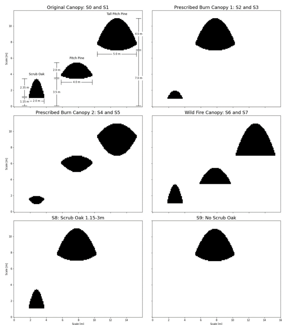
Figure 6. Visualization of woody vegetation parameterization for scenarios S0–S9.
