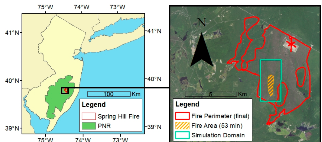
Figure 1. Spring Hill Fire location in the PNR (left). Spring fire perimeter at 53 min following ignition (estimated from time of detection), final fire perimeter, QUIC-Fire simulation domain (right).
