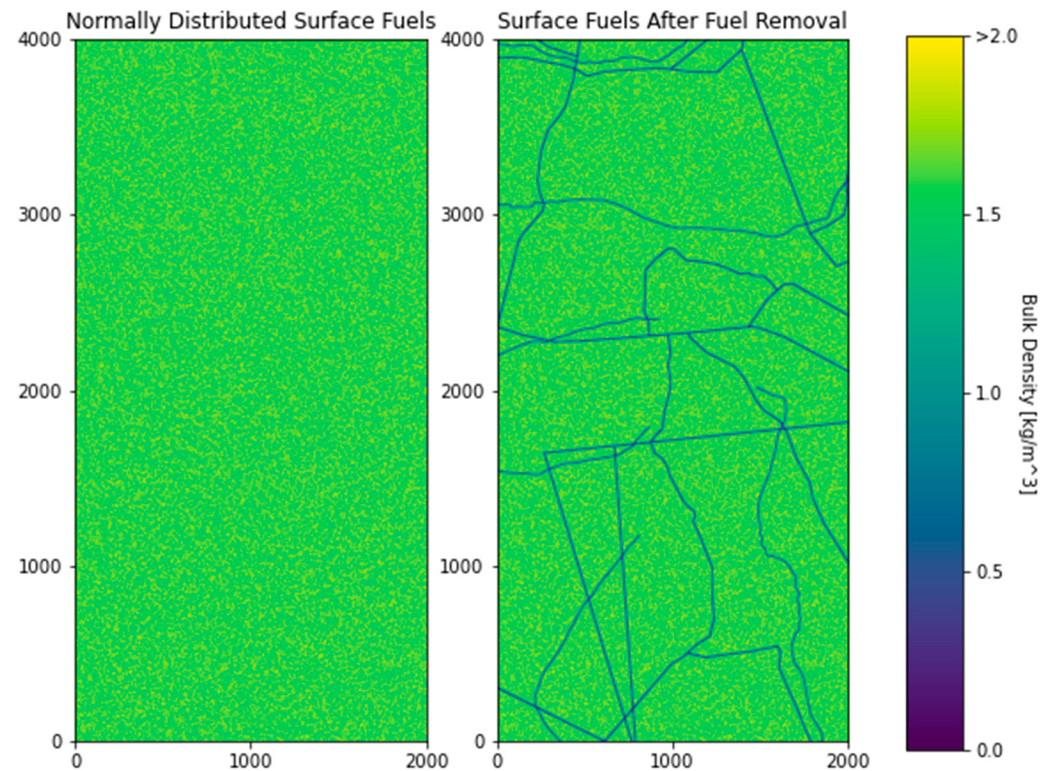
Figure 3. Bulk density of 1 m-tall surface fuel cells before and after fuel break removal.
