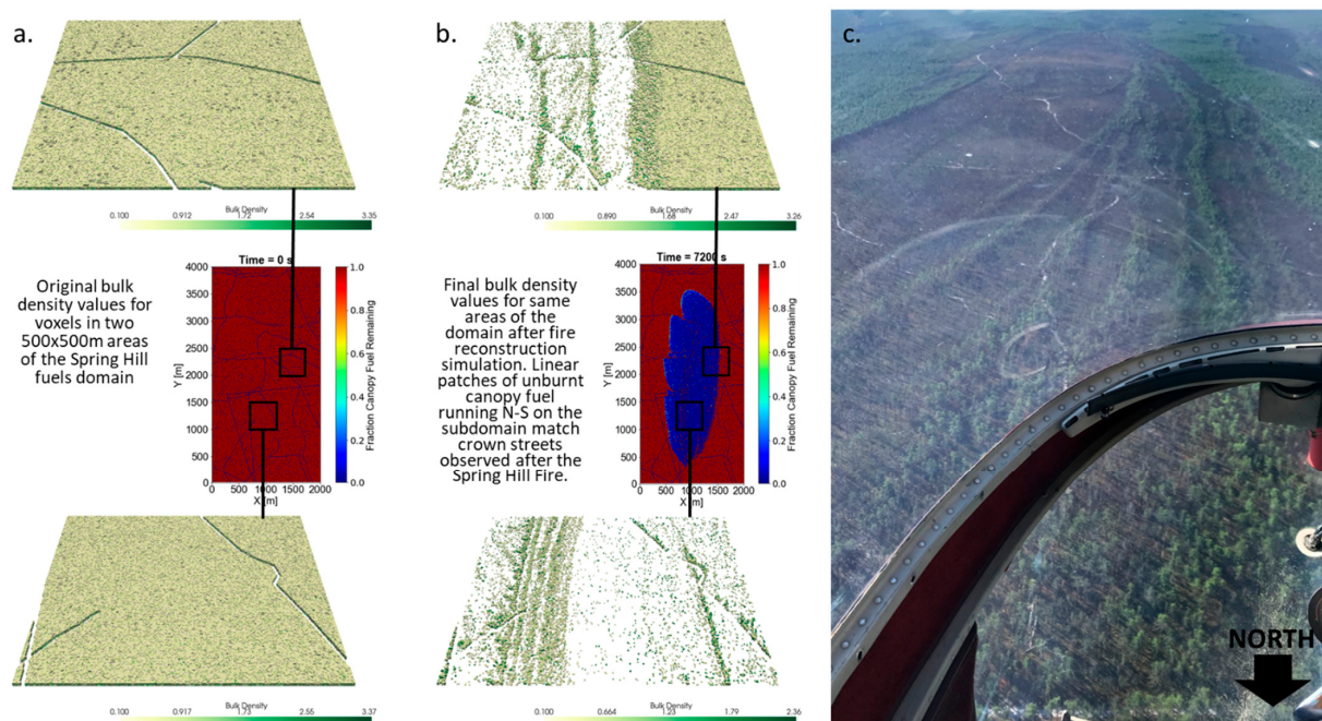
Figure A1. Tree crown streets, or long linear patterns of unburnt trees, were produced by the Spring Hill Fire reconstruction: (a,b) closely matched those observed following the actual fire (c). 3D renderings of QUIC-Fire outputs were created using the Python Pyvista library [50].
