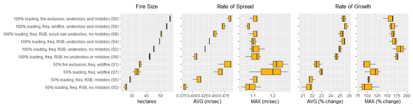
Figure 8. Fire size, rate of spread, and rate of growth results for 10 simulation scenarios differing in prior wildfire and prescribed fire management histories and fuel loading. Boxes refer to 1st–3rd quartile, thick vertical lines within boxes refer to median, and whiskers indicate minimum and maximum values of data distributions.
