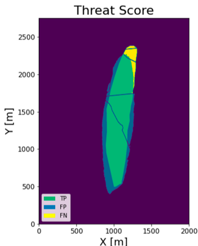
Figure 7. Visualization of threat score analysis comparing the simulated fire footprint to the field estimated burn plot 1 h after initial ignition. The green area represents the true positives, while the blue and yellow regions denote false positive and false negatives.
