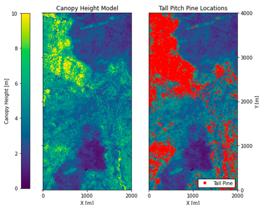
Figure 2. Canopy height and distribution of tall trees across the Spring Hill Fire domain.
