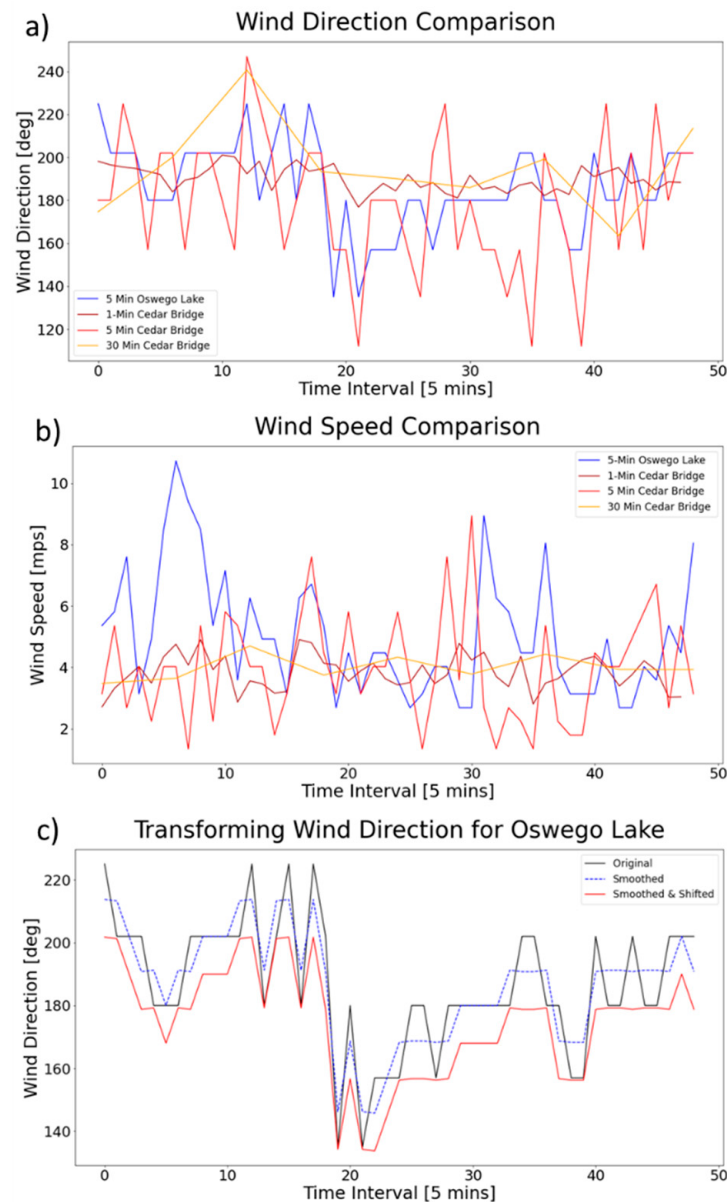
Figure 4. (a) Comparison of wind direction data collected at Oswego Lake and Cedar Bridge during the initial four hours of the Spring Hill Fire, (b) comparison of wind speed data collected at Oswego Lake and Cedar Bridge during the initial four hours of the Spring Hill Fire, and (c) transformations of Oswego Lake’s wind direction data. Original data was smoothed to reduce the dramatic fluctuations in direction due to low reporting precision of direction in the raw data.
