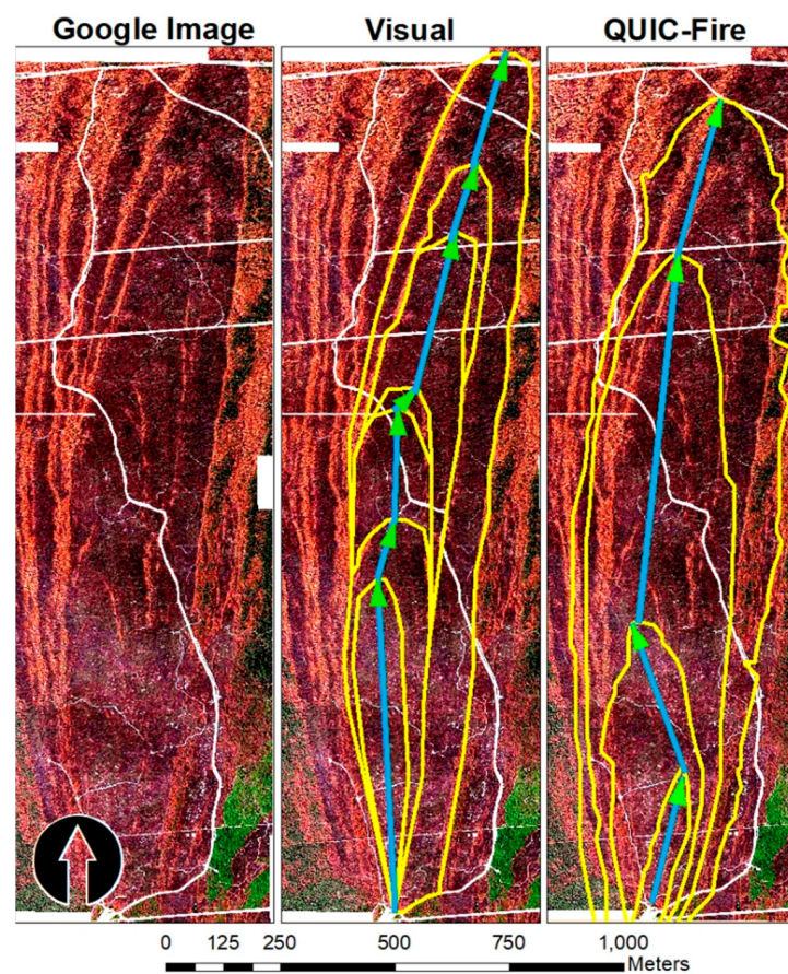
Figure 5. Comparison of visually estimated fire path of progression based on fire suppression staff observations and patterns in tree crown streets visible in post-fire Google imagery, and QUIC-Fire estimated progression (e.g., simulation scenario S0).
