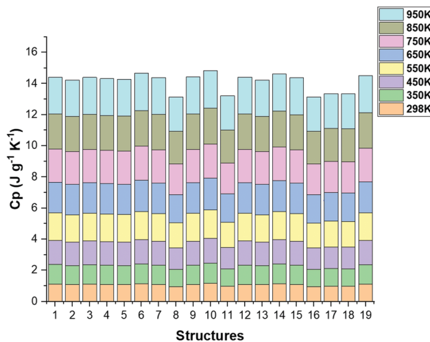
Fig. 8 Constant pressure heat capacity values for all structures in the current study at selected temperature. Structures 1–9 belong to product 1 starting from 1-mer to 9-mer with uniform increment in repeating unit. Similarly, structures 10–18 denote structures of varying sizes for product 2. Structure 19 denotes the reactant structure.
