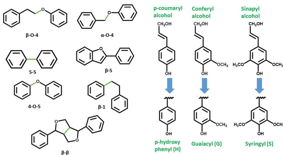
Fig. 1 Common linkages (left) and major monolignols (right) found in lignin.
