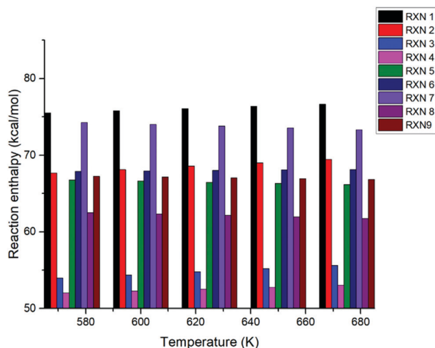
Fig. 4 BDE values for the homolytic \beta -O-4' cleavage reaction in hardwood model lignin decamer at different positions under selected temperature range of primary pyrolysis.
