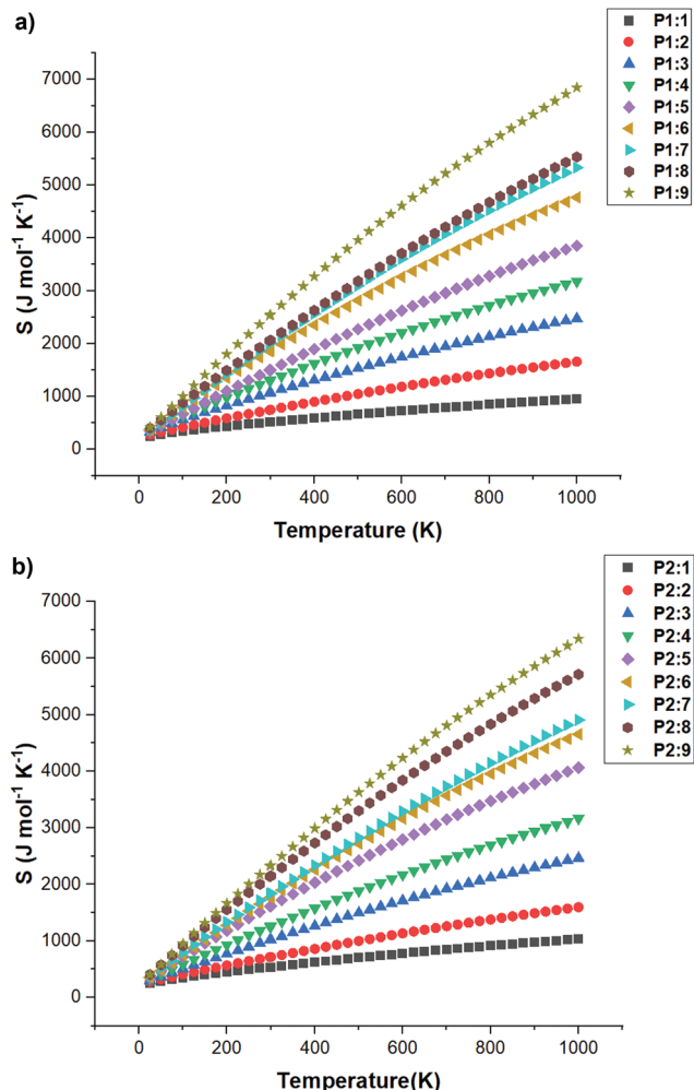
Fig. 10 (a) Entropy variation as a function of temperature for product 1 structures. Product 1 structures are phenoxyl radicals and denoted as P1. The number after this notation indicates the number of monomers present in each of these structures. (b) Entropy variation as a function of temperature for product 2 structures. Product 2 structures are C free radicals and denoted as P2. The number after this notation indicates the number of monomers present in each of these structures.
