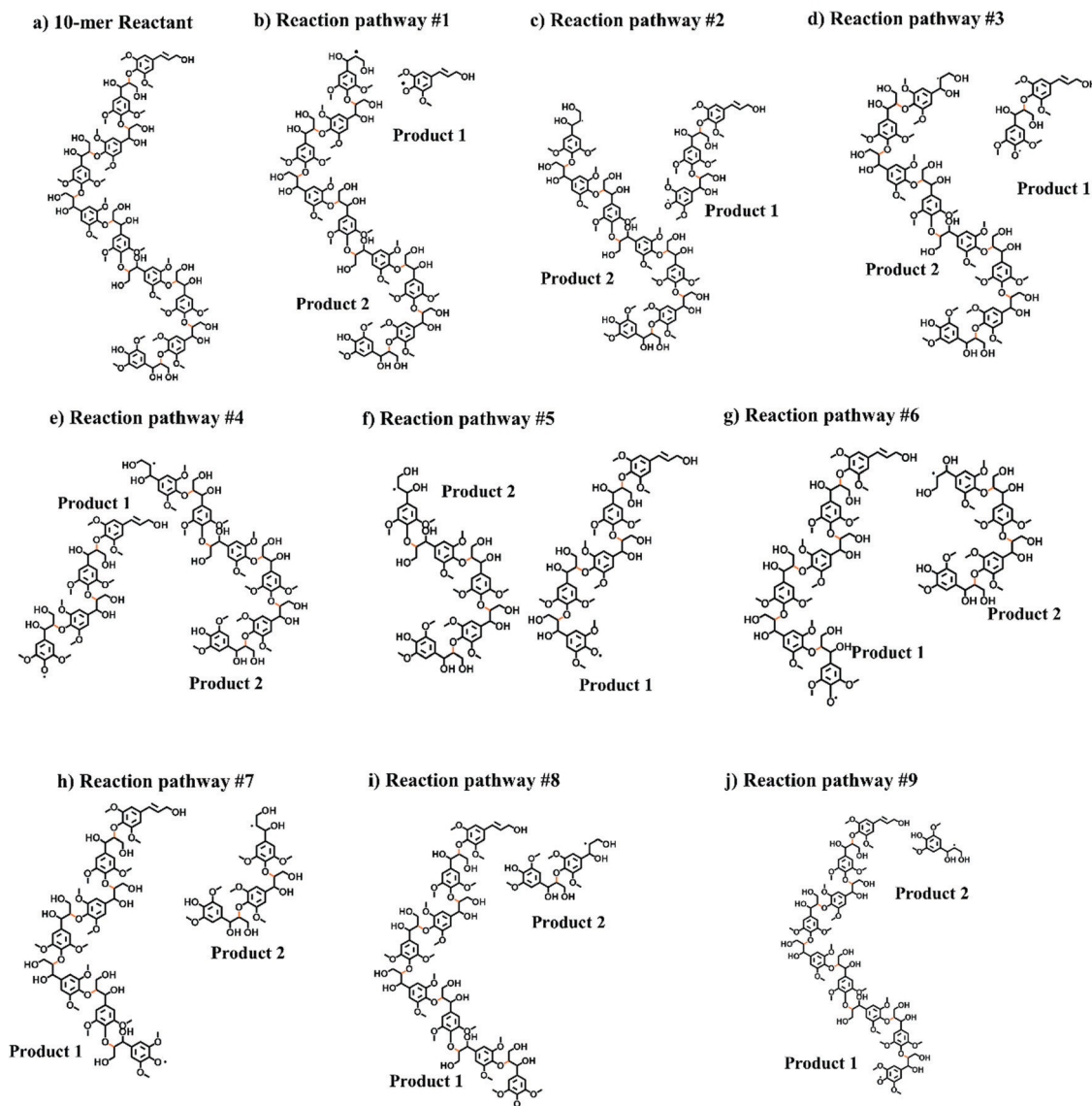
Fig. 2 (a) Initial reactant structure; (b–j) pairs of radical products generated along each of the nine reaction pathways for studying BDE of \beta -O-4' in model lignin oligomer. Products 1 and 2 are radical fragments with the radical center on oxygen and carbon atoms, respectively.
