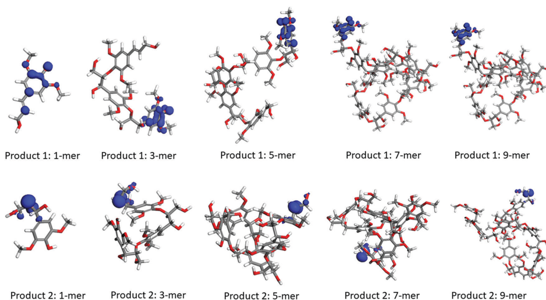
Fig. 7 Spin density plots with iso-value of 0.03 for selected free radical species studied in this work.
