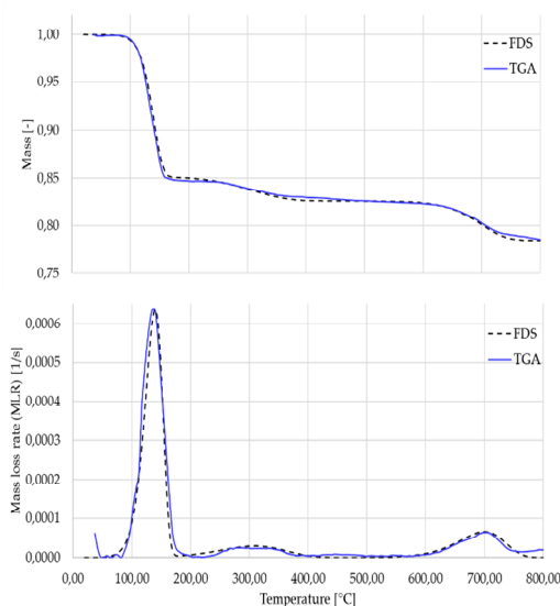
Fig. 6: TGA analysis in FDS and TGA measurement results comparison.
