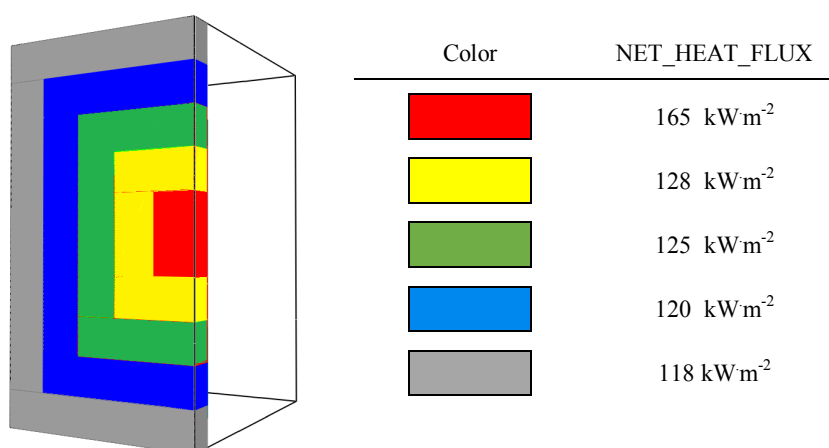
Fig. 4: H-TRIS panel model.
