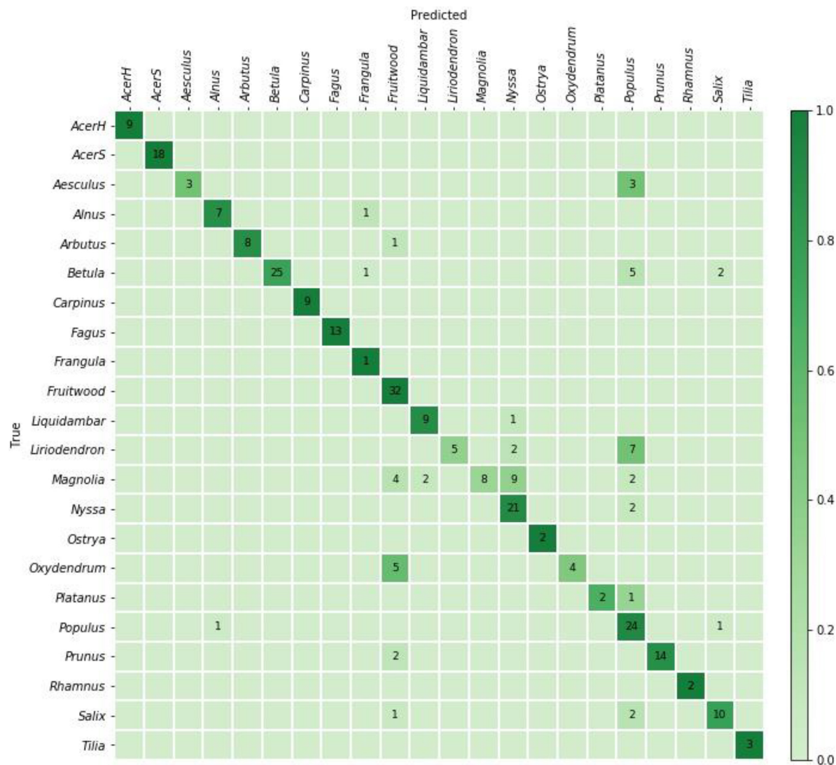
FIGURE 4 | Confusion matrix for the field model predictions on 284 PACw specimens. The top-1 and top-2 specimen-level accuracies were 80.6 and 90.5%, respectively.
