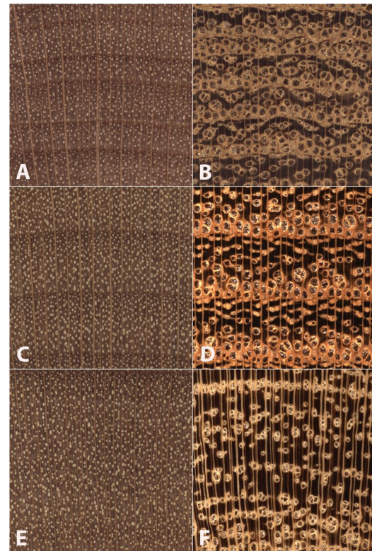
FIGURE 1 | Images of transverse surfaces of Betula alleghaniensis ( A,C,E ) and Robinia pseudoacacia ( B,D,F ) showing similar slow-growth conditions ( A,B ) medium-growth conditions ( C,D ), and faster-growth conditions ( E,F ). Note that Betula alleghaniensis shows comparatively lesser wood anatomical spatial heterogeneity than Robinia pseudoacacia . The nearly three complete growth rings in panels ( C,D ) present wood anatomical detail sufficient to facilitate an identification. The slow growth in panels ( A,B ) and partial growth rings in panels ( E,F ) demonstrate the comparatively lesser spatial heterogeneity of the diffuse porous Betula alleghaniensis . In Robinia pseudoacacia there is a lack of latewood characters in the slow-grown image ( B ), and only latewood anatomy in panel ( F ). By contrast, Betula alleghaniensis shows substantially similar anatomy across the three images ( A,C,E ).
