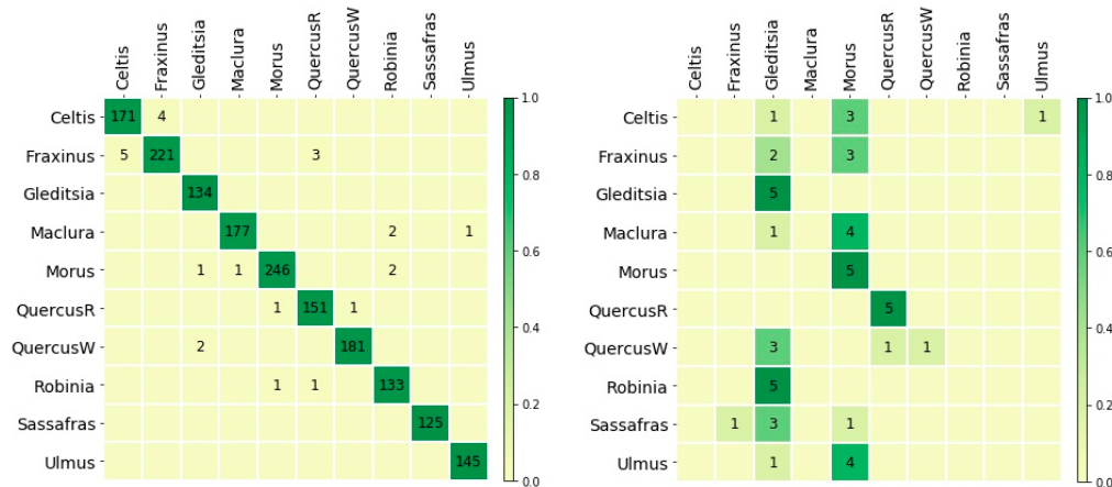
Figure 4. Confusion matrices for models trained on LD-train. (Left) Image-level confusion matrix for LD5. The confusion matrix, and accuracy (98.5%), were obtained by aggregating over the five cross-validation folds. (Right) specimen-level confusion matrix for LDF on LD-test images with an accuracy of 32.0%. The only classes with correct predictions were Gleditsia, Morus, QuercusR, and QuercusW.
