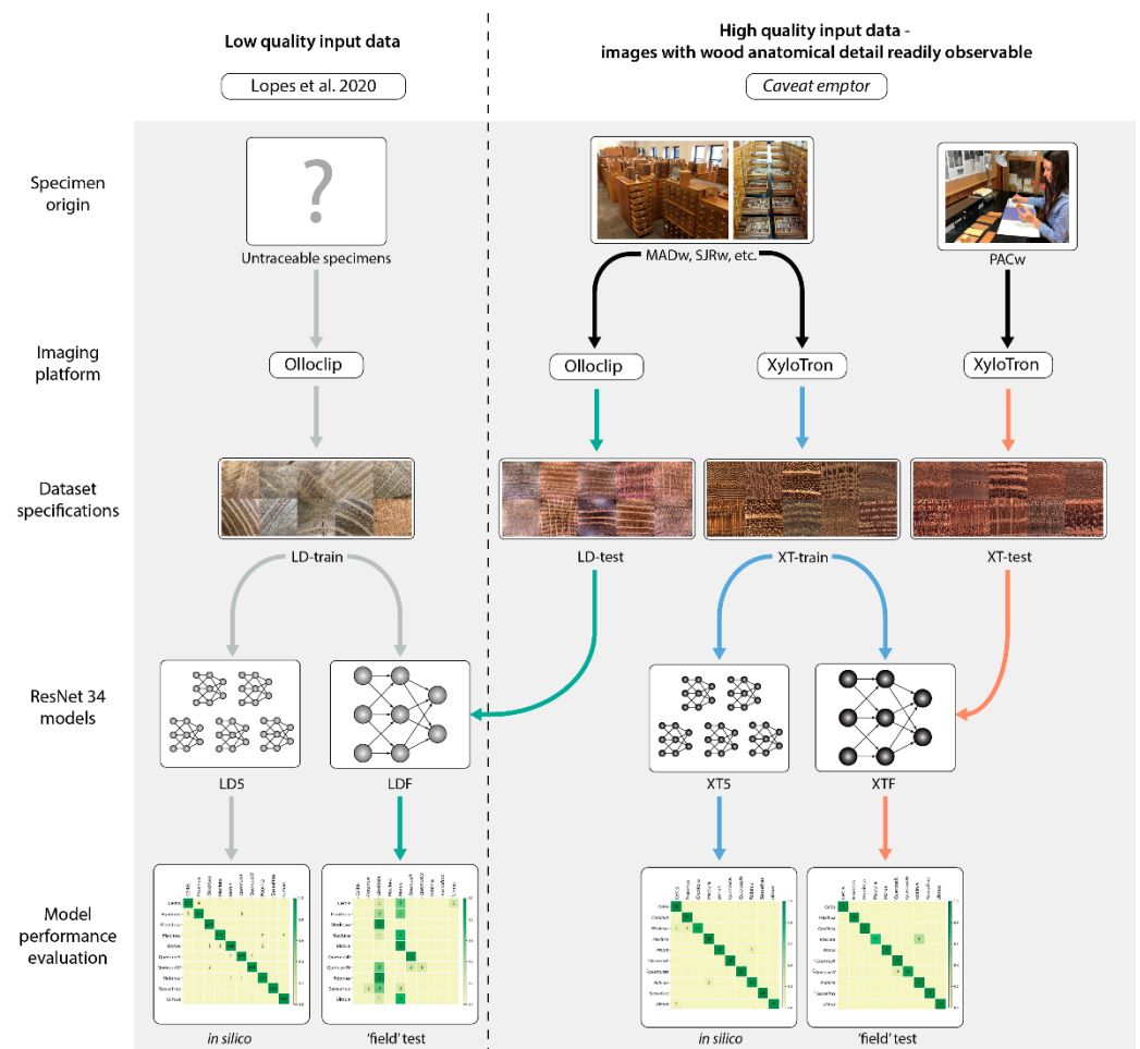
Figure 3. A schematic of the project workflow and the relationships between datasets, models, and evaluations.
