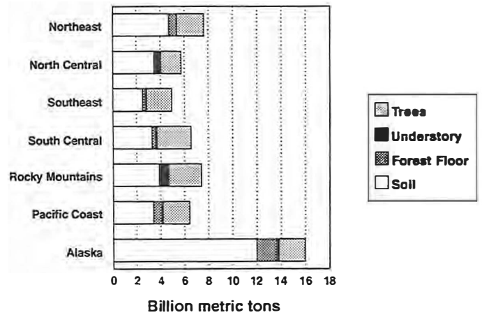
Figure 4.2.—Total carbon storage by region and ecosystem component, U.S. forests, 1992.
