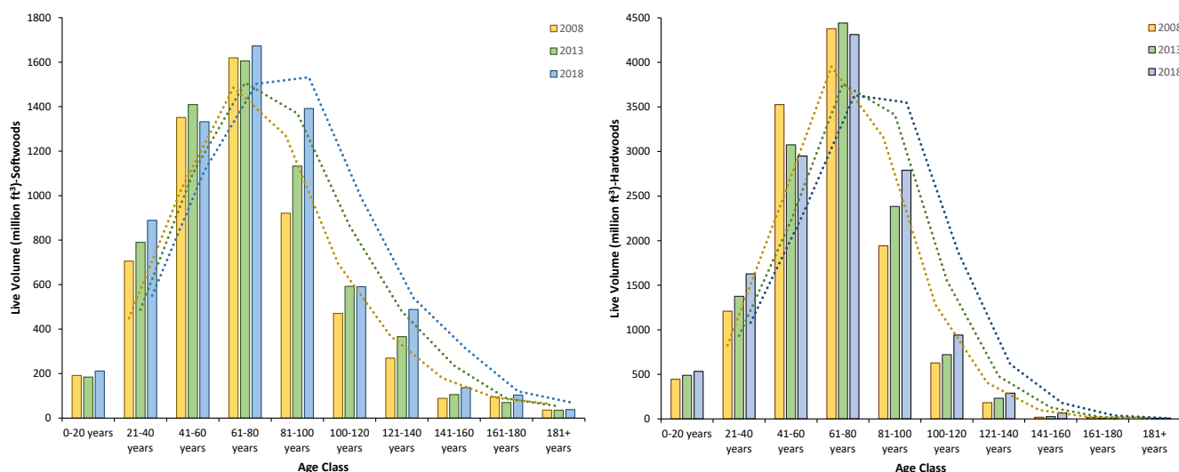
Figure 6. —Softwood (A) and hardwood (B) volume by inventory year and age class on forest land. Dotted lines represent two-class moving average, Minnesota. Note the scale on the y axis is different in the two graphs.
